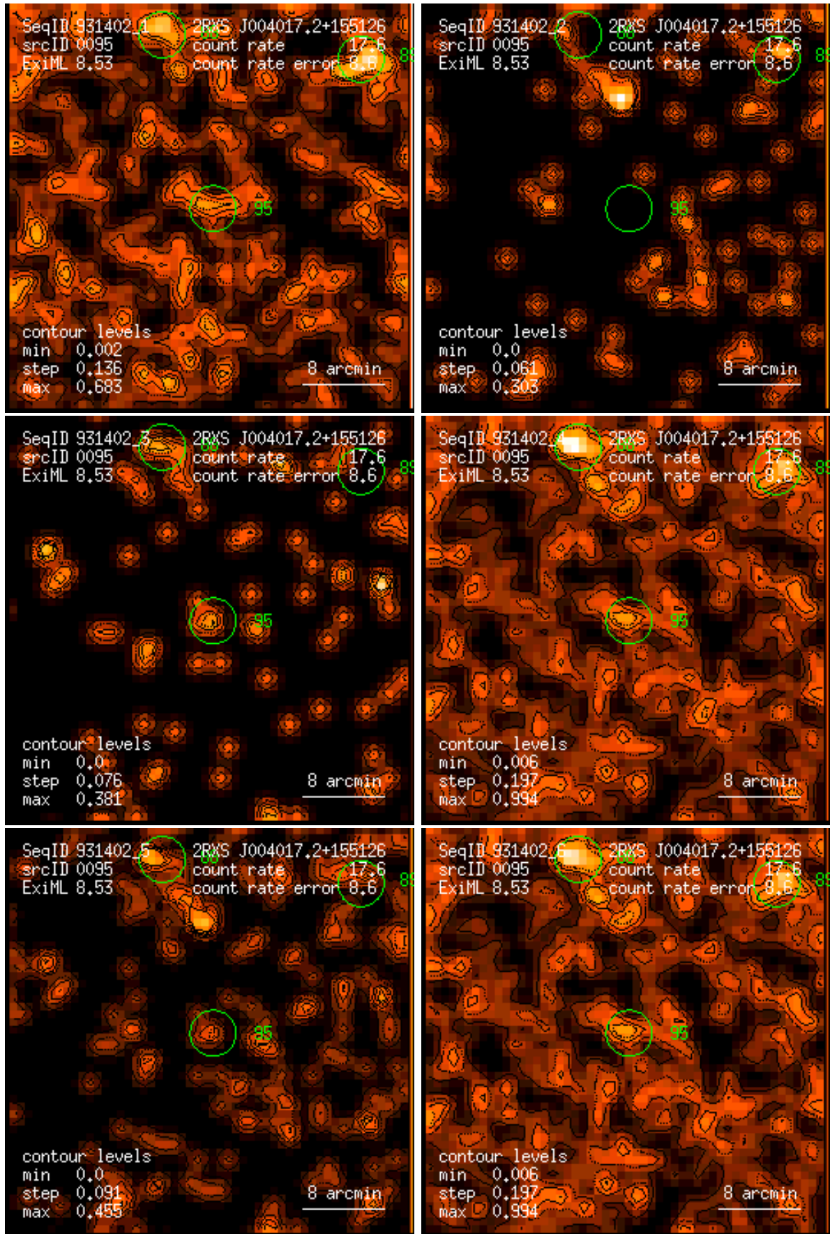
Figure 95: RASS 931402: detection 0095: band rate images, Gaussian filter: (1) PSPC channels 11 – 41, (2) 52 – 90, (3) 91 – 201, (4) 11 – 235, (5) 52 – 201, (6) 11 – 201. Broad band rates in counts/ks. Band rate contour levels in counts/ks/arcmin 2 .
