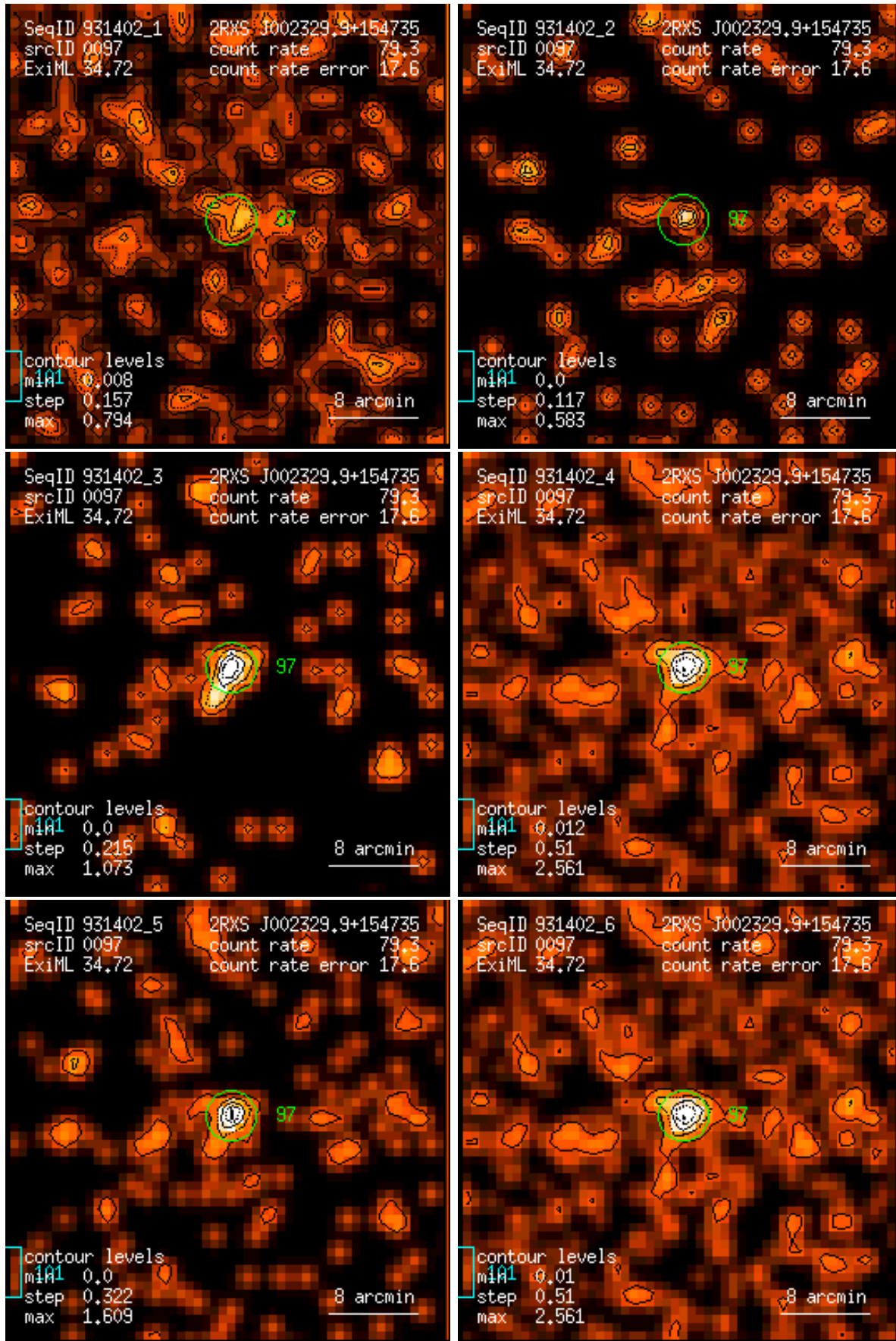
Figure 97: RASS 931402: detection 0097: band rate images, Gaussian filter: (1) PSPC channels 11 – 41, (2) 52 – 90, (3) 91 – 201, (4) 11 – 235, (5) 52 – 201, (6) 11 – 201. Broad band rates in counts/ks. Band rate contour levels in counts/ks/arcmin 2 .
