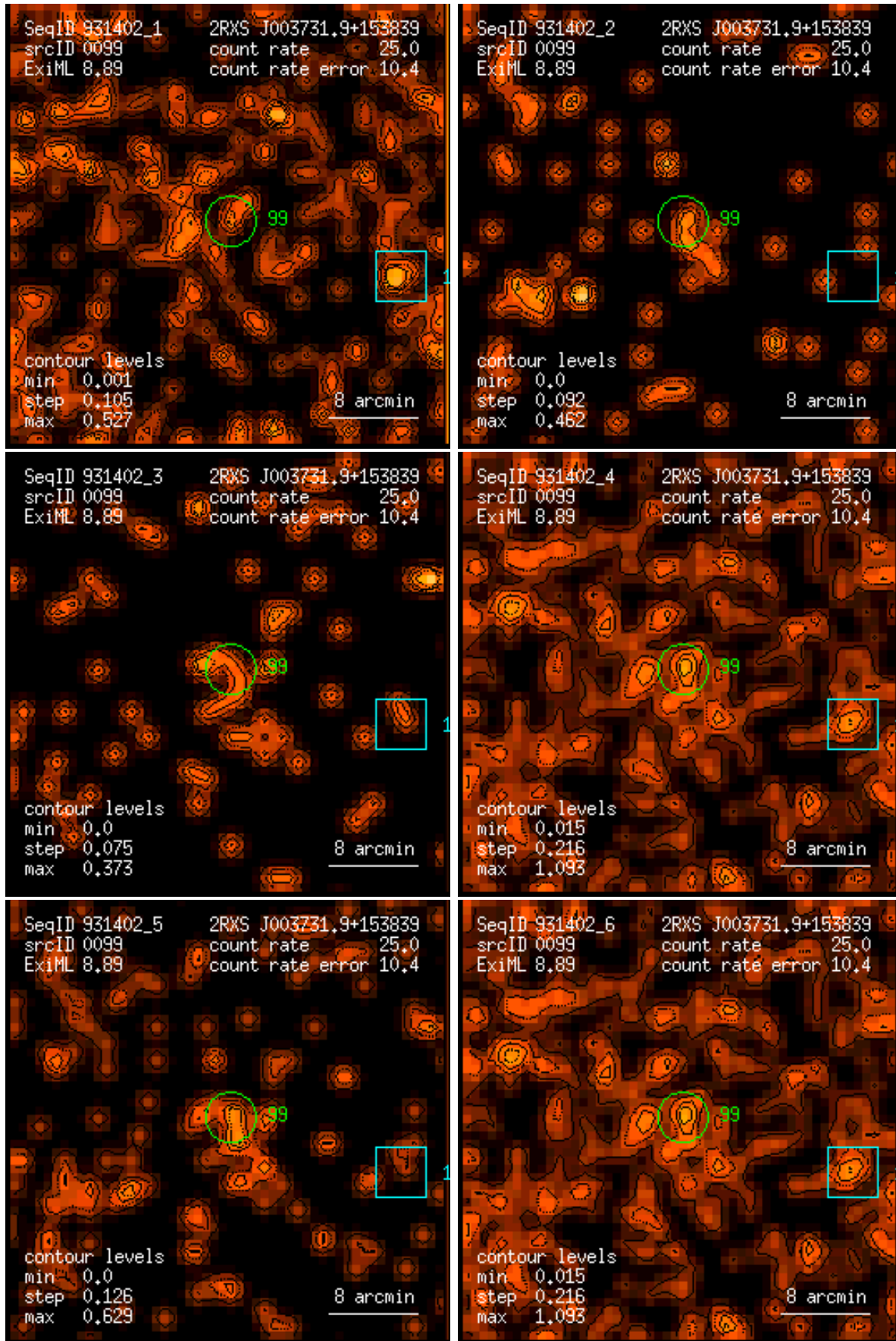
Figure 99: RASS 931402: detection 0099: band rate images, Gaussian filter: (1) PSPC channels 11 – 41, (2) 52 – 90, (3) 91 – 201, (4) 11 – 235, (5) 52 – 201, (6) 11 – 201. Broad band rates in counts/ks. Band rate contour levels in counts/ks/arcmin 2 .
