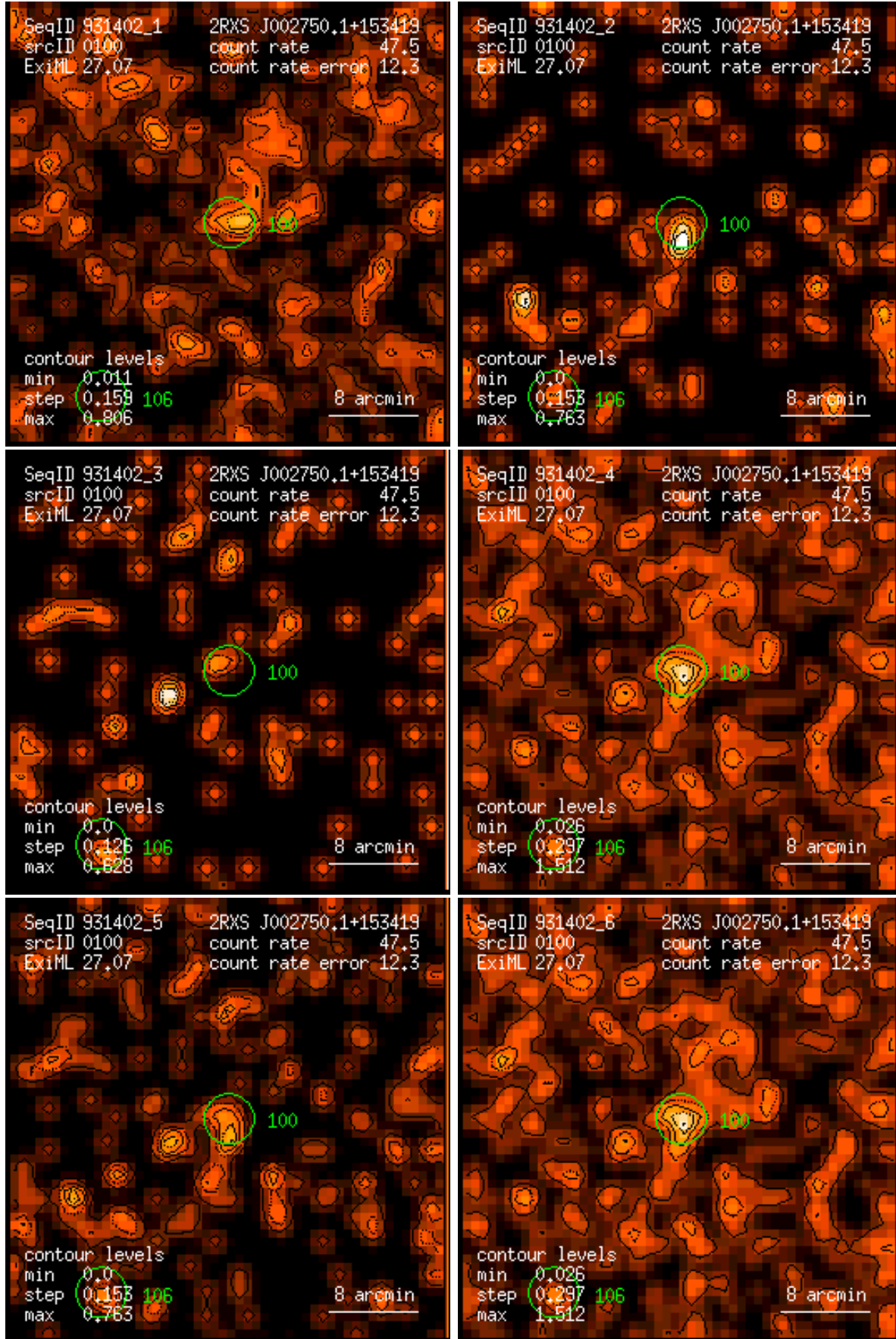
Figure 100: RASS 931402: detection 0100: band rate images, Gaussian filter: (1) PSPC channels 11 – 41, (2) 52 – 90, (3) 91 – 201, (4) 11 – 235, (5) 52 – 201, (6) 11 – 201. Broad band rates in counts/ks. Band rate contour levels in counts/ks/arcmin 2 .
