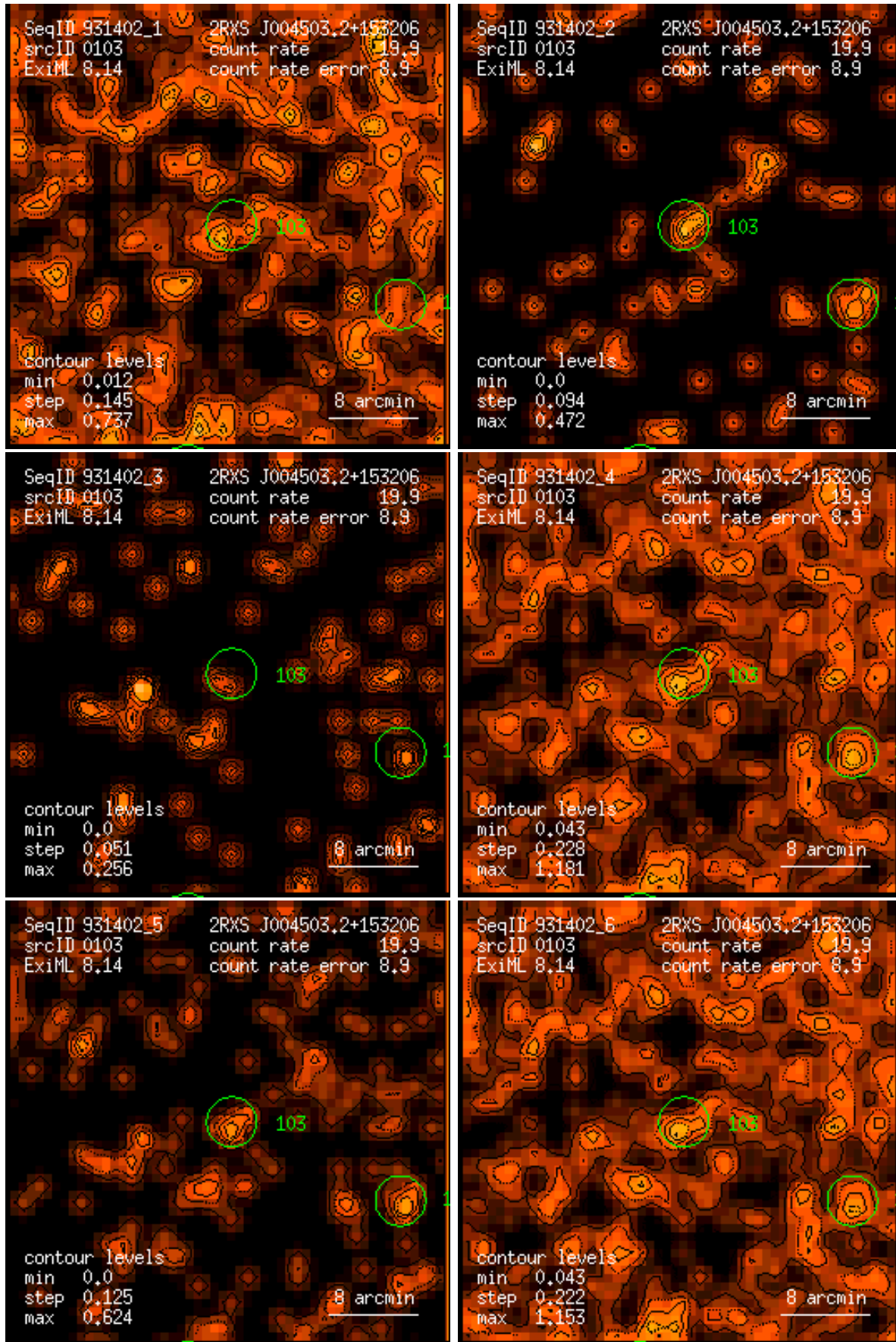
Figure 103: RASS 931402: detection 0103: band rate images, Gaussian filter: (1) PSPC channels 11 – 41, (2) 52 – 90, (3) 91 – 201, (4) 11 – 235, (5) 52 – 201, (6) 11 – 201. Broad band rates in counts/ks. Band rate contour levels in counts/ks/arcmin 2 .
