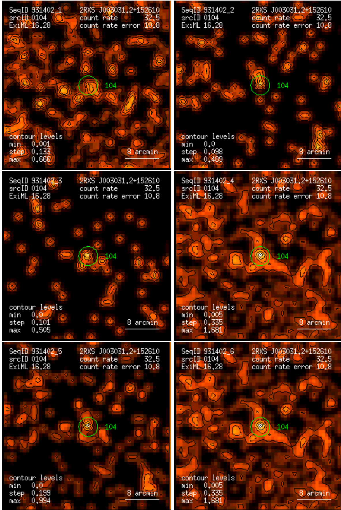
Figure 104: RASS 931402: detection 0104: band rate images, Gaussian filter: (1) PSPC channels 11 – 41, (2) 52 – 90, (3) 91 – 201, (4) 11 – 235, (5) 52 – 201, (6) 11 – 201. Broad band rates in counts/ks. Band rate contour levels in counts/ks/arcmin 2 .
