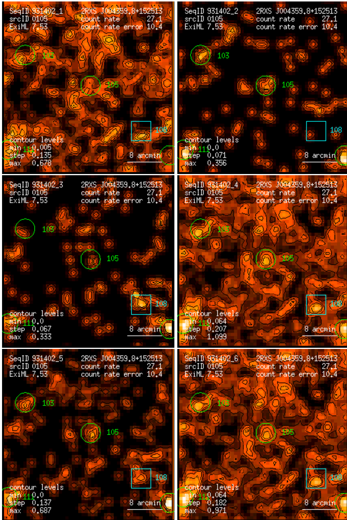
Figure 105: RASS 931402: detection 0105: band rate images, Gaussian filter: (1) PSPC channels 11 – 41, (2) 52 – 90, (3) 91 – 201, (4) 11 – 235, (5) 52 – 201, (6) 11 – 201. Broad band rates in counts/ks. Band rate contour levels in counts/ks/arcmin 2 .
