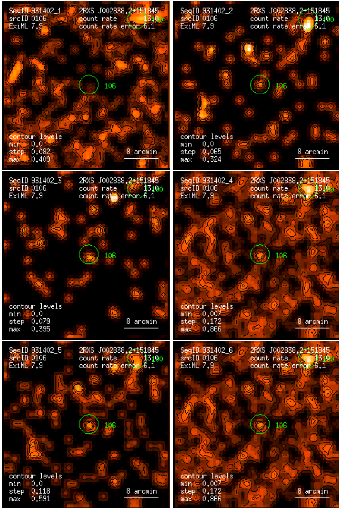
Figure 106: RASS 931402: detection 0106: band rate images, Gaussian filter: (1) PSPC channels 11 – 41, (2) 52 – 90, (3) 91 – 201, (4) 11 – 235, (5) 52 – 201, (6) 11 – 201. Broad band rates in counts/ks. Band rate contour levels in counts/ks/arcmin 2 .
