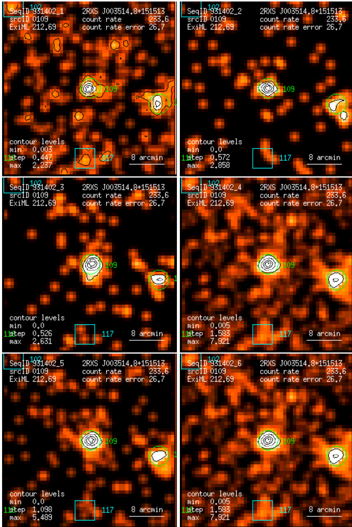
Figure 109: RASS 931402: detection 0109: band rate images, Gaussian filter: (1) PSPC channels 11 – 41, (2) 52 – 90, (3) 91 – 201, (4) 11 – 235, (5) 52 – 201, (6) 11 – 201. Broad band rates in counts/ks. Band rate contour levels in counts/ks/arcmin 2 .
