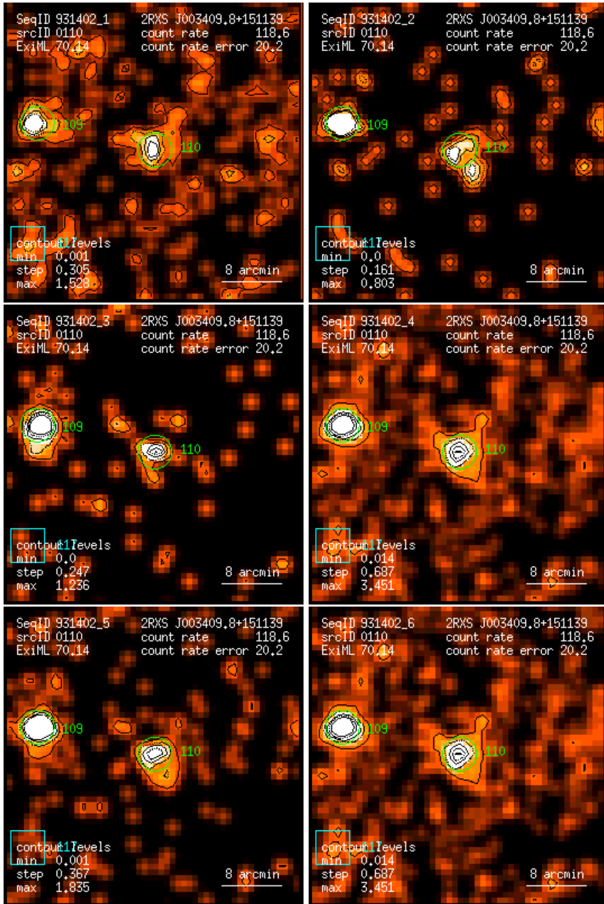
Figure 110: RASS 931402: detection 0110: band rate images, Gaussian filter: (1) PSPC channels 11 – 41, (2) 52 – 90, (3) 91 – 201, (4) 11 – 235, (5) 52 – 201, (6) 11 – 201. Broad band rates in counts/ks. Band rate contour levels in counts/ks/arcmin 2 .
