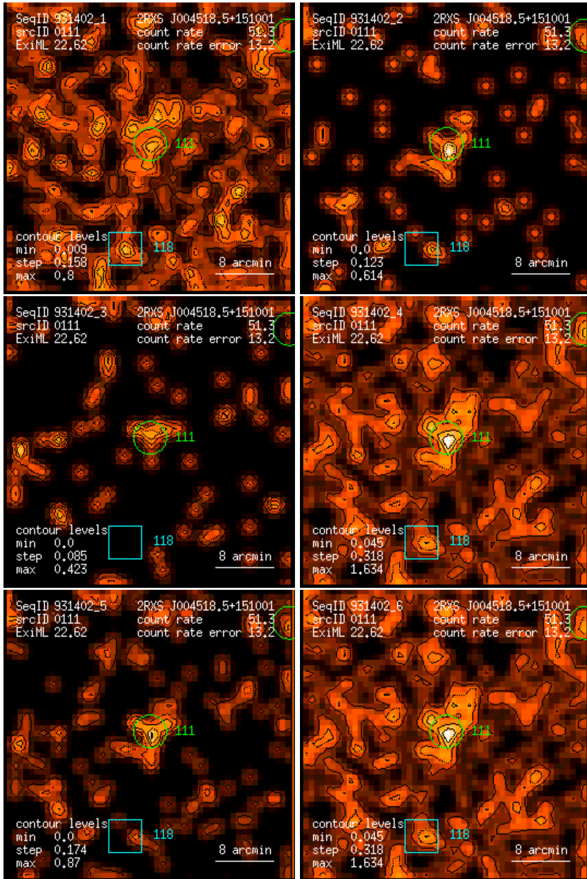
Figure 111: RASS 931402: detection 0111: band rate images, Gaussian filter: (1) PSPC channels 11 – 41, (2) 52 – 90, (3) 91 – 201, (4) 11 – 235, (5) 52 – 201, (6) 11 – 201. Broad band rates in counts/ks. Band rate contour levels in counts/ks/arcmin 2 .
