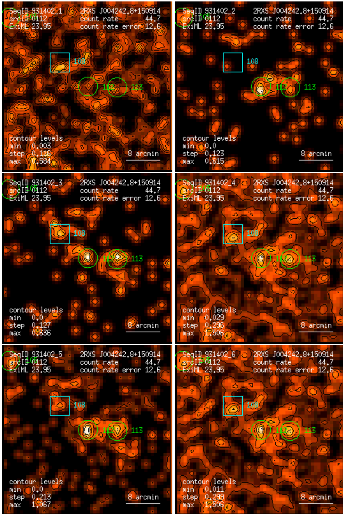
Figure 112: RASS 931402: detection 0112: band rate images, Gaussian filter: (1) PSPC channels 11 – 41, (2) 52 – 90, (3) 91 – 201, (4) 11 – 235, (5) 52 – 201, (6) 11 – 201. Broad band rates in counts/ks. Band rate contour levels in counts/ks/arcmin 2 .
