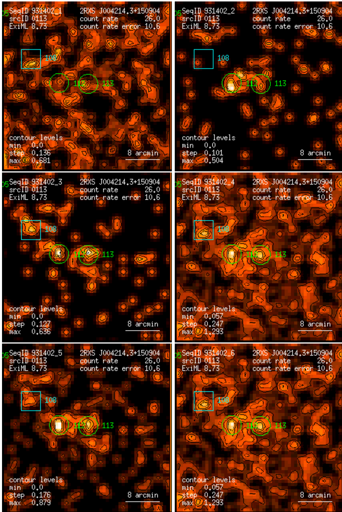
Figure 113: RASS 931402: detection 0113: band rate images, Gaussian filter: (1) PSPC channels 11 – 41, (2) 52 – 90, (3) 91 – 201, (4) 11 – 235, (5) 52 – 201, (6) 11 – 201. Broad band rates in counts/ks. Band rate contour levels in counts/ks/arcmin 2 .
