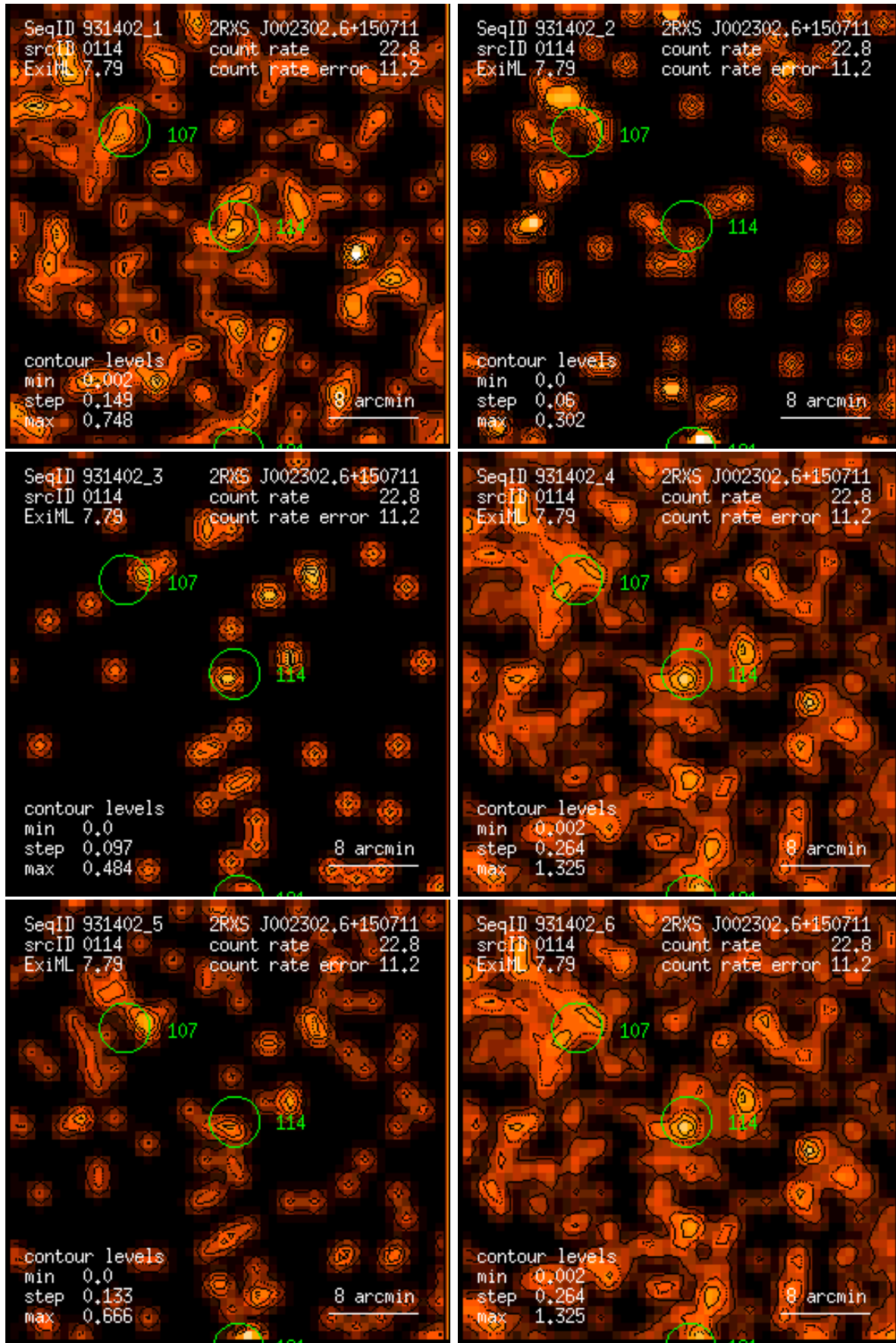
Figure 114: RASS 931402: detection 0114: band rate images, Gaussian filter: (1) PSPC channels 11 – 41, (2) 52 – 90, (3) 91 – 201, (4) 11 – 235, (5) 52 – 201, (6) 11 – 201. Broad band rates in counts/ks. Band rate contour levels in counts/ks/arcmin 2 .
