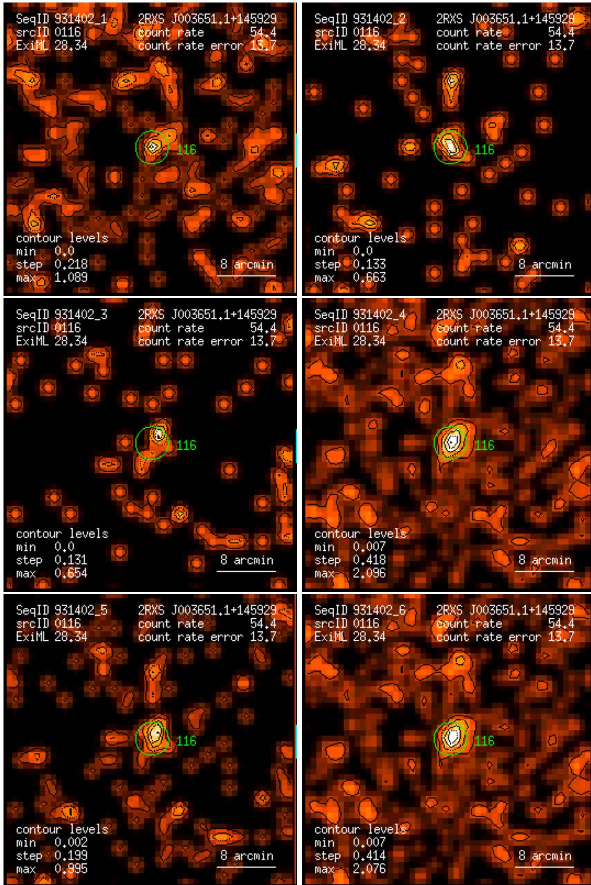
Figure 116: RASS 931402: detection 0116: band rate images, Gaussian filter: (1) PSPC channels 11 – 41, (2) 52 – 90, (3) 91 – 201, (4) 11 – 235, (5) 52 – 201, (6) 11 – 201. Broad band rates in counts/ks. Band rate contour levels in counts/ks/arcmin 2 .
