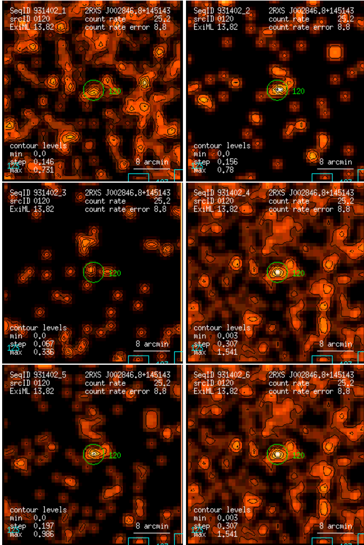
Figure 120: RASS 931402: detection 0120: band rate images, Gaussian filter: (1) PSPC channels 11 – 41, (2) 52 – 90, (3) 91 – 201, (4) 11 – 235, (5) 52 – 201, (6) 11 – 201. Broad band rates in counts/ks. Band rate contour levels in counts/ks/arcmin 2 .
