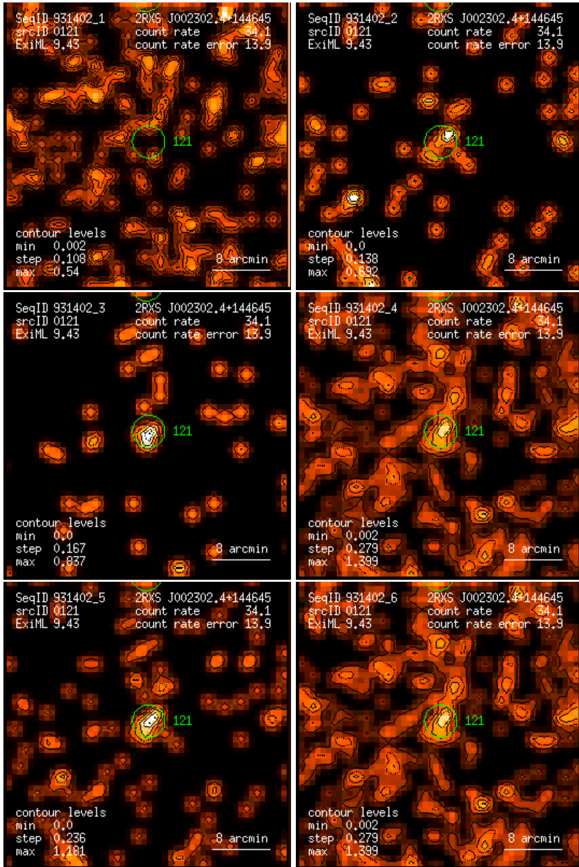
Figure 121: RASS 931402: detection 0121: band rate images, Gaussian filter: (1) PSPC channels 11 – 41, (2) 52 – 90, (3) 91 – 201, (4) 11 – 235, (5) 52 – 201, (6) 11 – 201. Broad band rates in counts/ks. Band rate contour levels in counts/ks/arcmin 2 .
