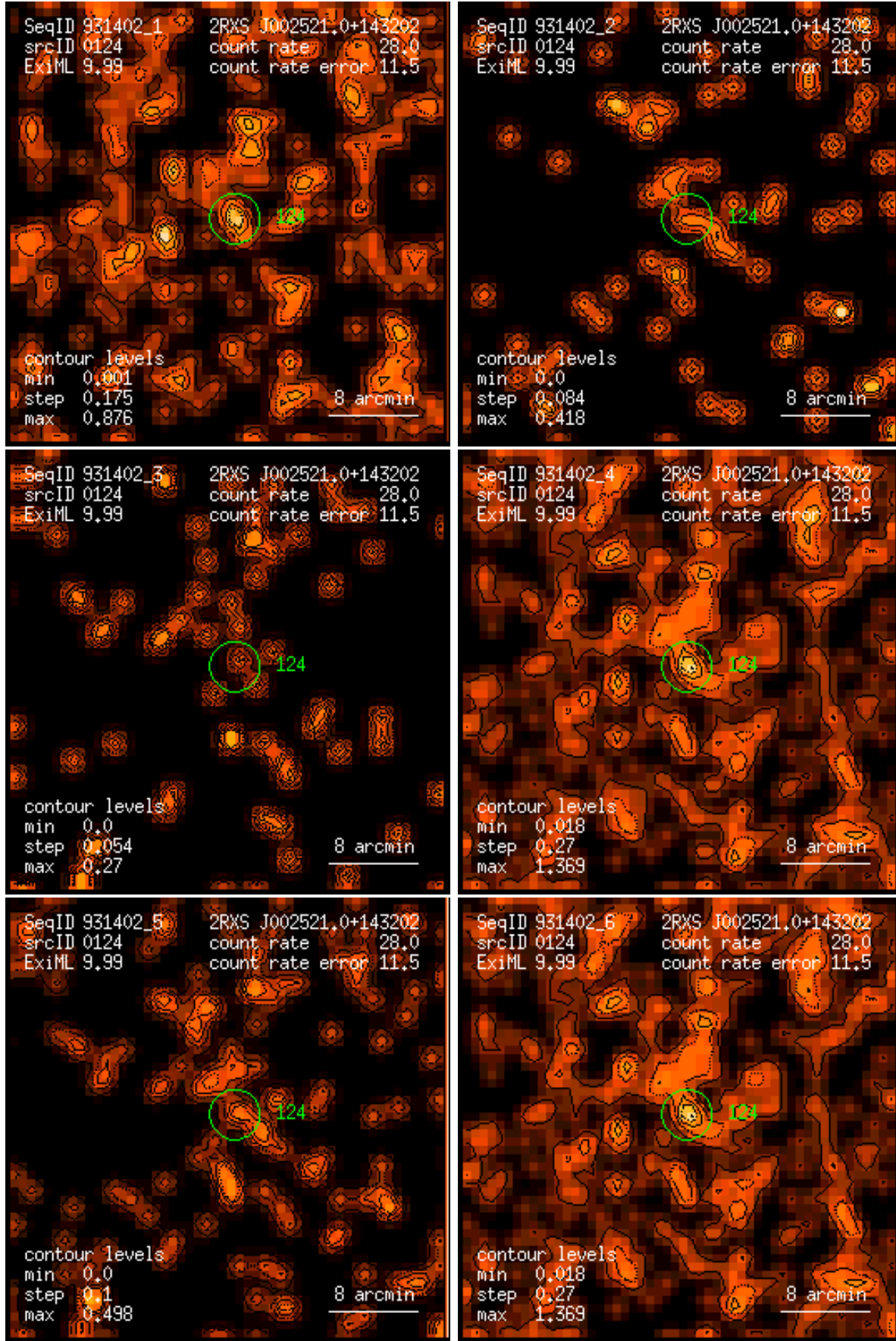
Figure 124: RASS 931402: detection 0124: band rate images, Gaussian filter: (1) PSPC channels 11 – 41, (2) 52 – 90, (3) 91 – 201, (4) 11 – 235, (5) 52 – 201, (6) 11 – 201. Broad band rates in counts/ks. Band rate contour levels in counts/ks/arcmin 2 .
