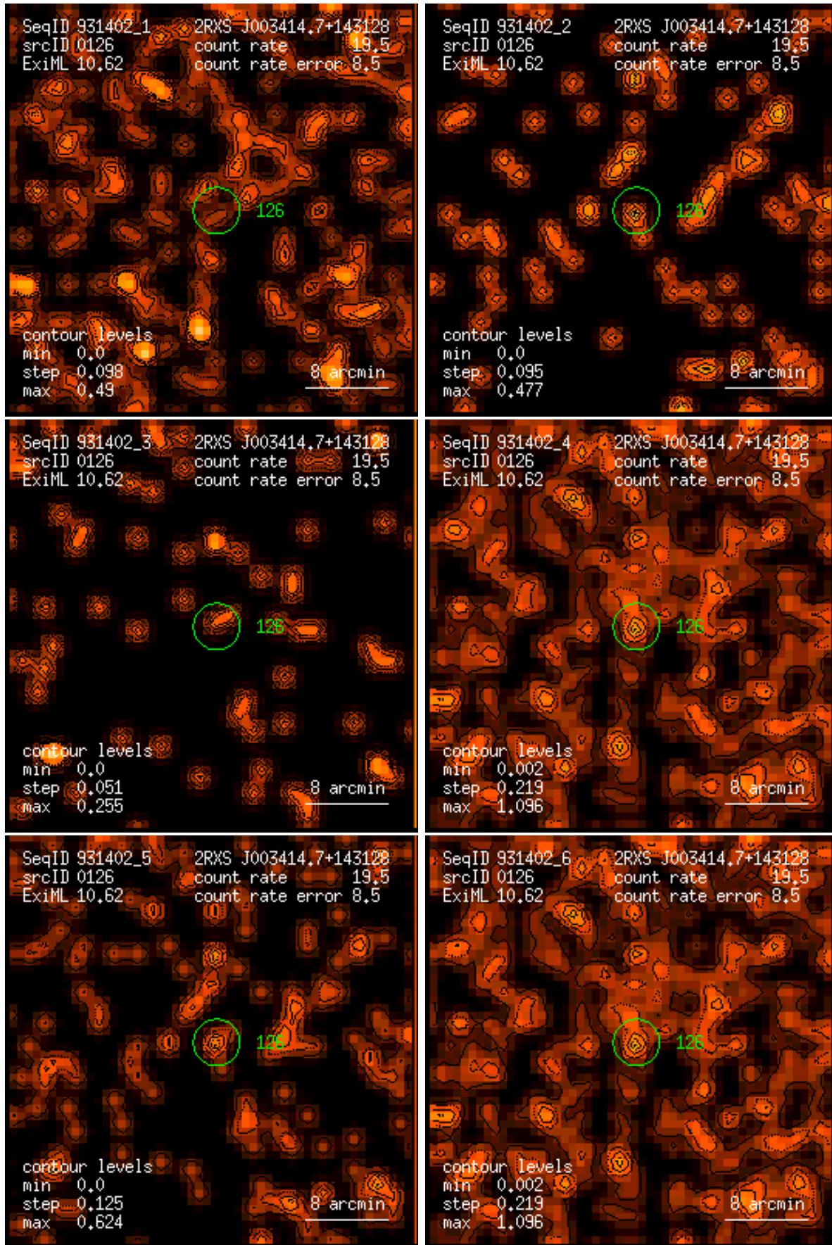
Figure 126: RASS 931402: detection 0126: band rate images, Gaussian filter: (1) PSPC channels 11 – 41, (2) 52 – 90, (3) 91 – 201, (4) 11 – 235, (5) 52 – 201, (6) 11 – 201. Broad band rates in counts/ks. Band rate contour levels in counts/ks/arcmin 2 .
