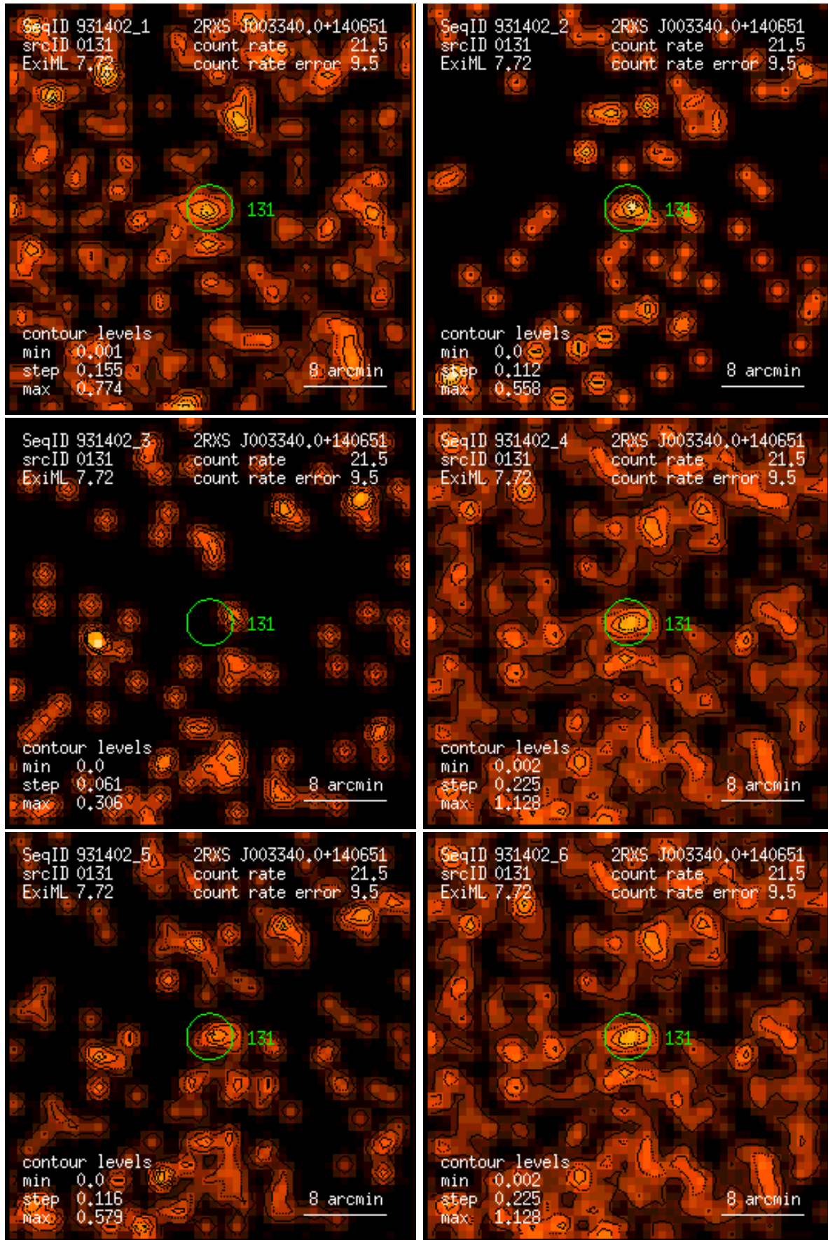
Figure 131: RASS 931402: detection 0131: band rate images, Gaussian filter: (1) PSPC channels 11 – 41, (2) 52 – 90, (3) 91 – 201, (4) 11 – 235, (5) 52 – 201, (6) 11 – 201. Broad band rates in counts/ks. Band rate contour levels in counts/ks/arcmin 2 .
