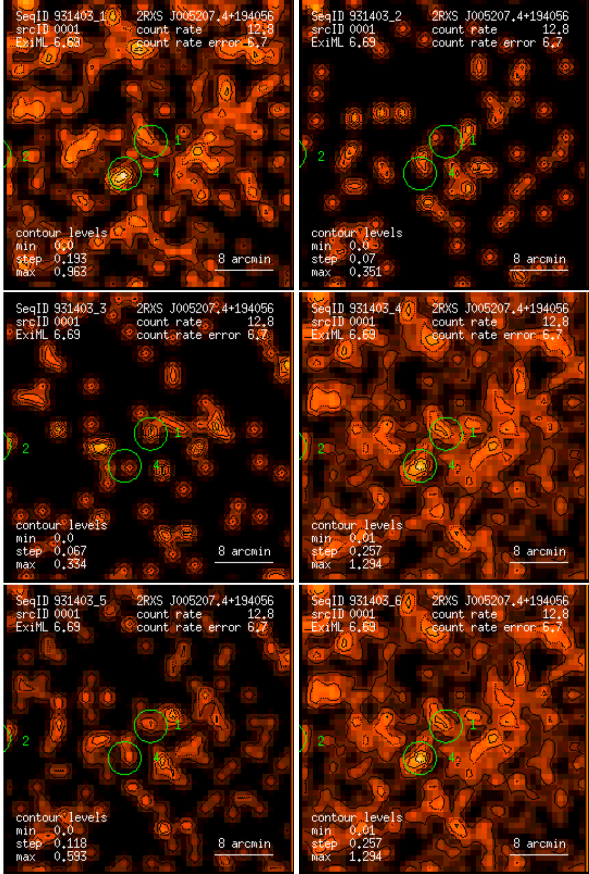
Figure 1: RASS 931403: detection 0001: band rate images, Gaussian filter: (1) PSPC channels 11 – 41, (2) 52 – 90, (3) 91 – 201, (4) 11 – 235, (5) 52 – 201, (6) 11 – 201. Broad band rates in counts/ks. Band rate contour levels in counts/ks/arcmin 2 .
