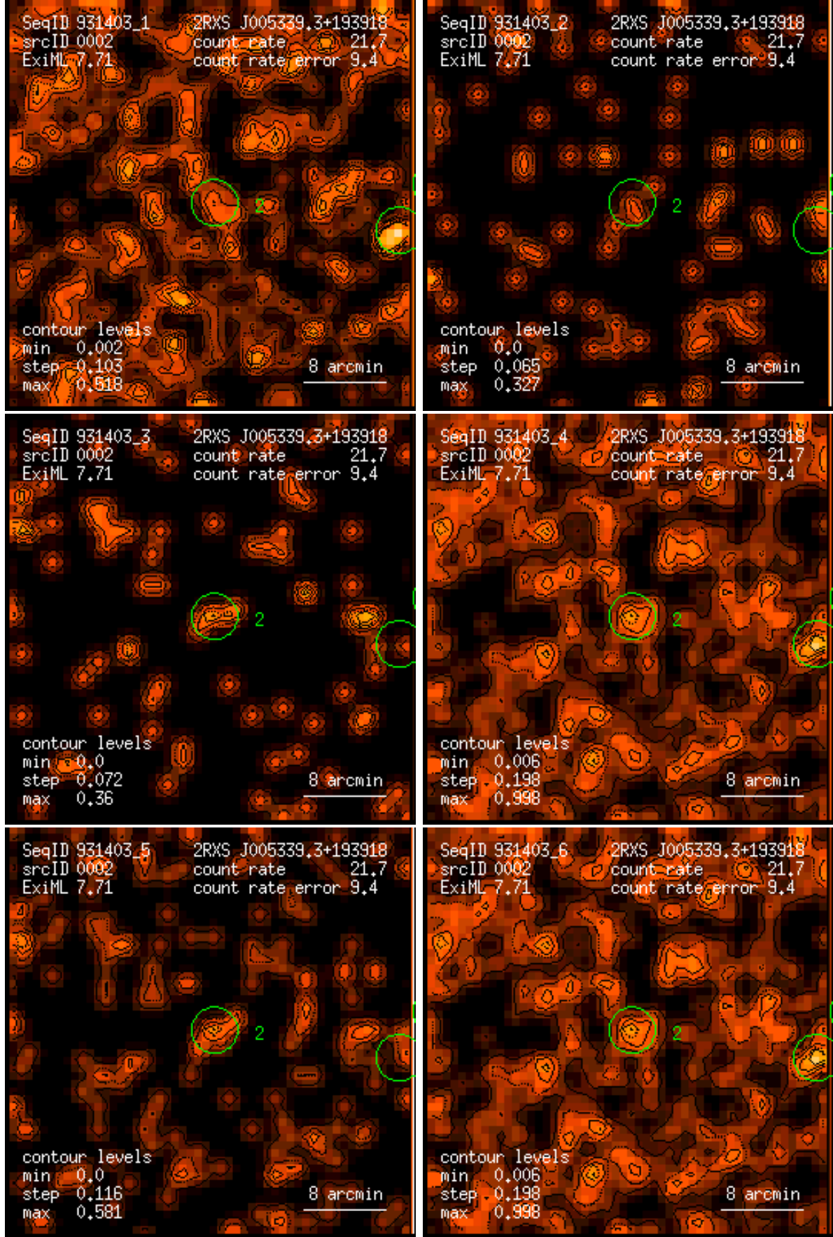
Figure 2: RASS 931403: detection 0002: band rate images, Gaussian filter: (1) PSPC channels 11 – 41, (2) 52 – 90, (3) 91 – 201, (4) 11 – 235, (5) 52 – 201, (6) 11 – 201. Broad band rates in counts/ks. Band rate contour levels in counts/ks/arcmin 2 .
