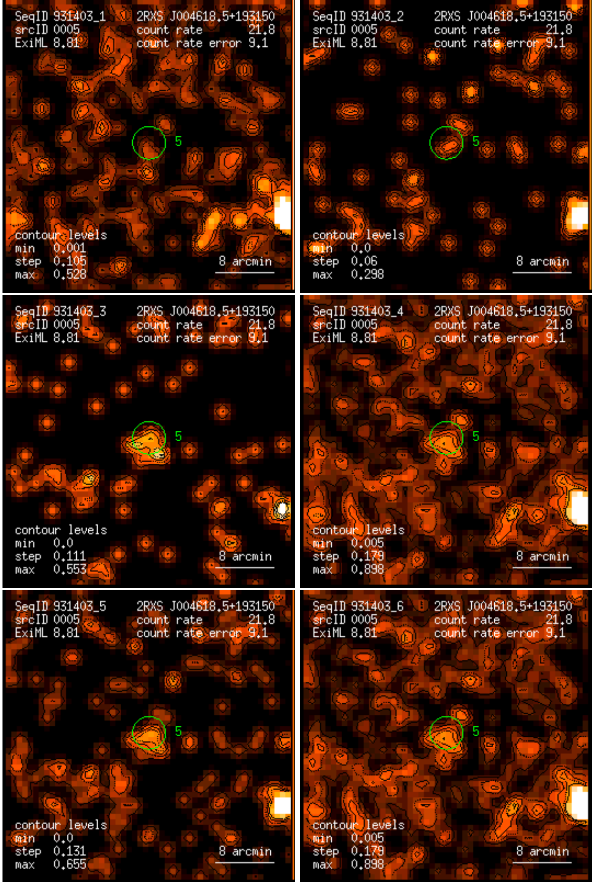
Figure 5: RASS 931403: detection 0005: band rate images, Gaussian filter: (1) PSPC channels 11 – 41, (2) 52 – 90, (3) 91 – 201, (4) 11 – 235, (5) 52 – 201, (6) 11 – 201. Broad band rates in counts/ks. Band rate contour levels in counts/ks/arcmin 2 .
