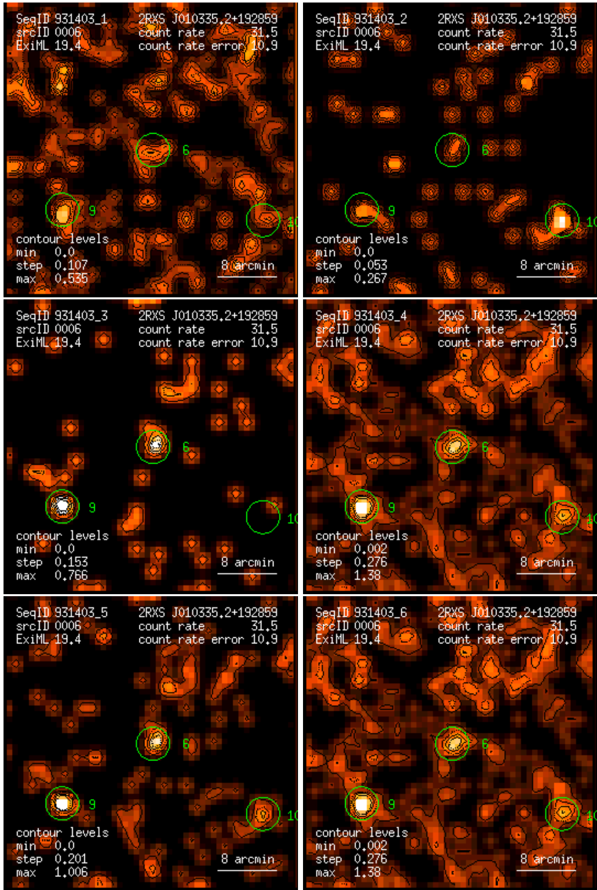
Figure 6: RASS 931403: detection 0006: band rate images, Gaussian filter: (1) PSPC channels 11 – 41, (2) 52 – 90, (3) 91 – 201, (4) 11 – 235, (5) 52 – 201, (6) 11 – 201. Broad band rates in counts/ks. Band rate contour levels in counts/ks/arcmin 2 .
