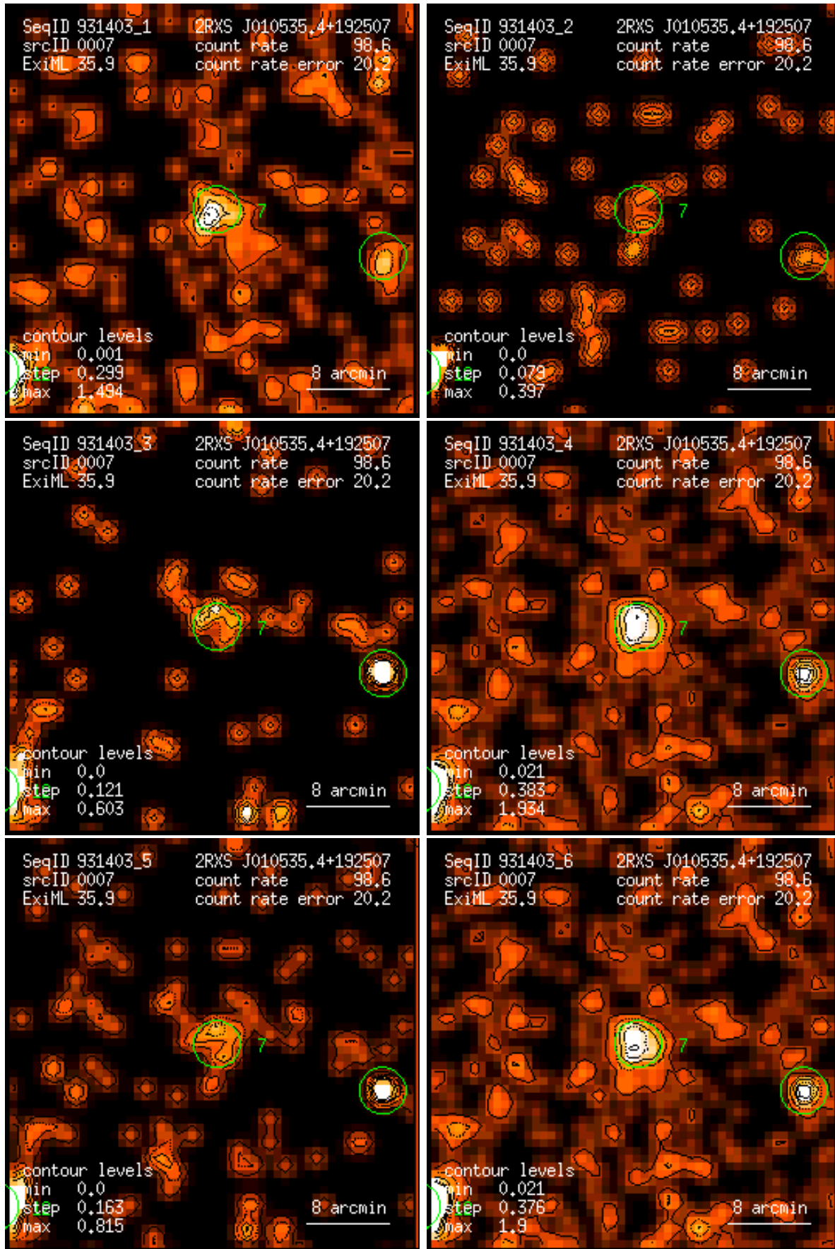
Figure 7: RASS 931403: detection 0007: band rate images, Gaussian filter: (1) PSPC channels 11 – 41, (2) 52 – 90, (3) 91 – 201, (4) 11 – 235, (5) 52 – 201, (6) 11 – 201. Broad band rates in counts/ks. Band rate contour levels in counts/ks/arcmin 2 .
