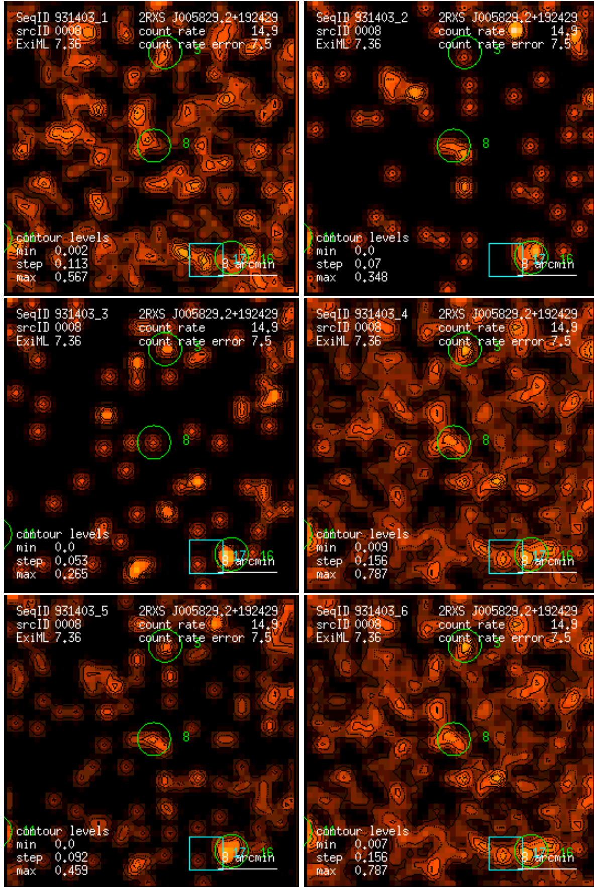
Figure 8: RASS 931403: detection 0008: band rate images, Gaussian filter: (1) PSPC channels 11 – 41, (2) 52 – 90, (3) 91 – 201, (4) 11 – 235, (5) 52 – 201, (6) 11 – 201. Broad band rates in counts/ks. Band rate contour levels in counts/ks/arcmin 2 .
