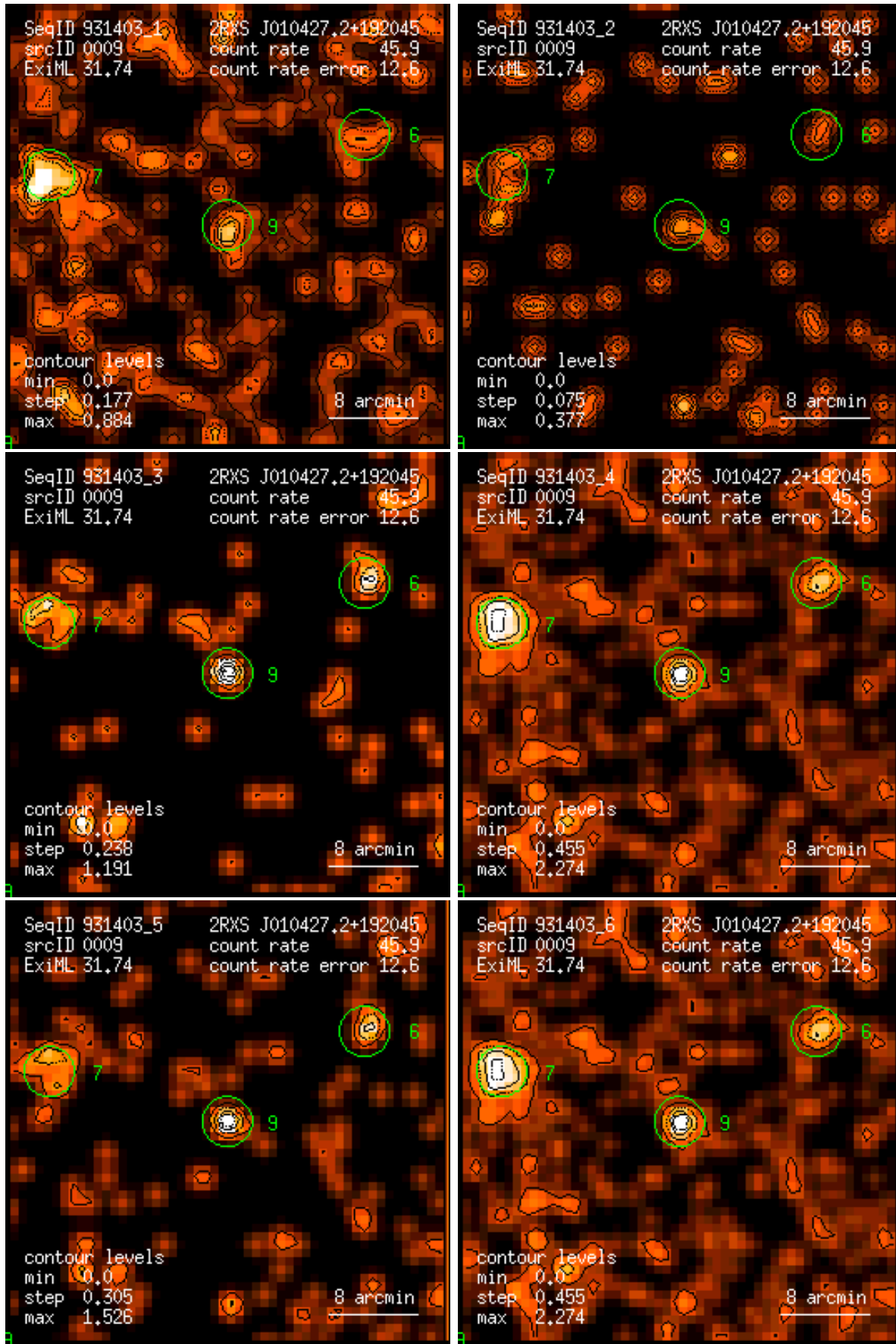
Figure 9: RASS 931403: detection 0009: band rate images, Gaussian filter: (1) PSPC channels 11 – 41, (2) 52 – 90, (3) 91 – 201, (4) 11 – 235, (5) 52 – 201, (6) 11 – 201. Broad band rates in counts/ks. Band rate contour levels in counts/ks/arcmin 2 .
