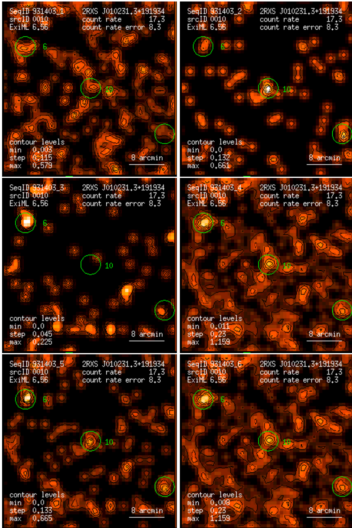
Figure 10: RASS 931403: detection 0010: band rate images, Gaussian filter: (1) PSPC channels 11 – 41, (2) 52 – 90, (3) 91 – 201, (4) 11 – 235, (5) 52 – 201, (6) 11 – 201. Broad band rates in counts/ks. Band rate contour levels in counts/ks/arcmin 2 .
