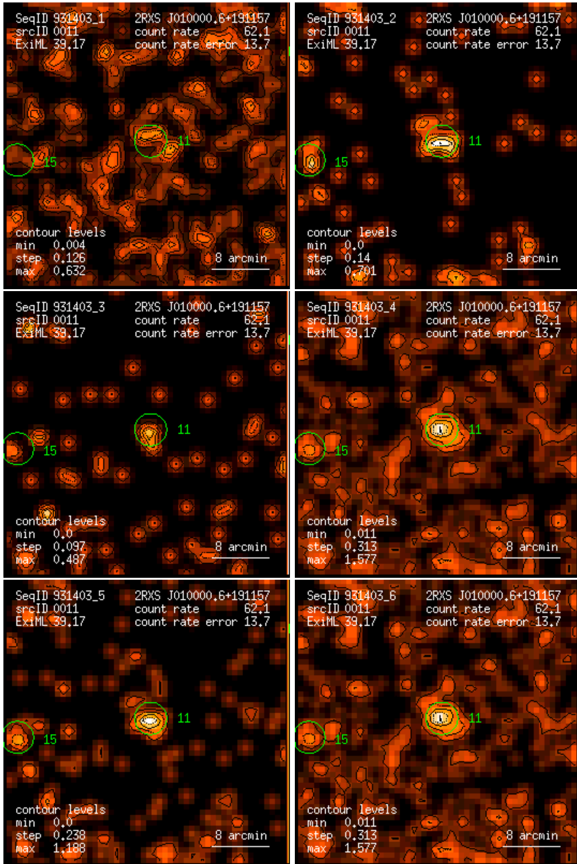
Figure 11: RASS 931403: detection 0011: band rate images, Gaussian filter: (1) PSPC channels 11 – 41, (2) 52 – 90, (3) 91 – 201, (4) 11 – 235, (5) 52 – 201, (6) 11 – 201. Broad band rates in counts/ks. Band rate contour levels in counts/ks/arcmin 2 .
