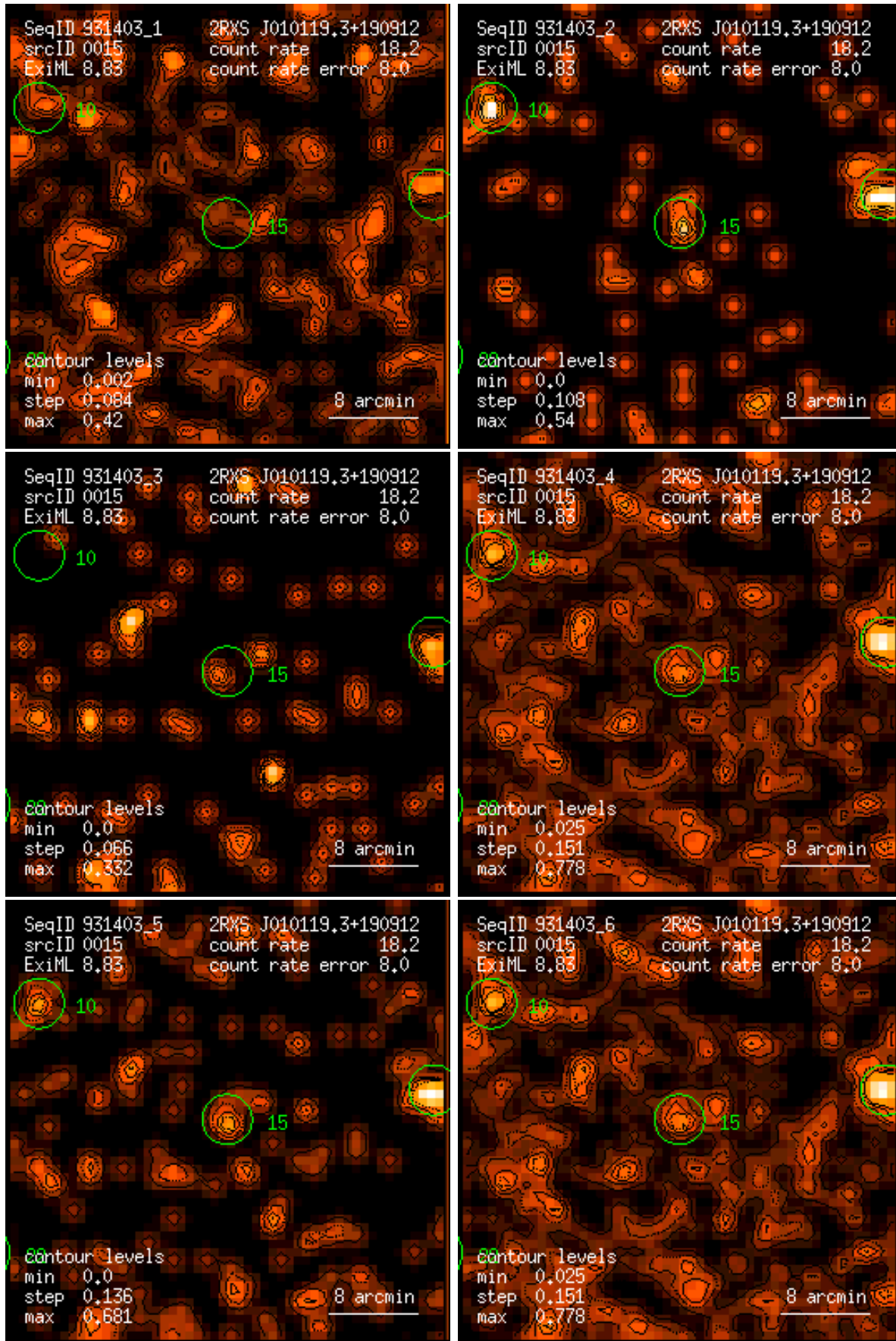
Figure 15: RASS 931403: detection 0015: band rate images, Gaussian filter: (1) PSPC channels 11 – 41, (2) 52 – 90, (3) 91 – 201, (4) 11 – 235, (5) 52 – 201, (6) 11 – 201. Broad band rates in counts/ks. Band rate contour levels in counts/ks/arcmin 2 .
