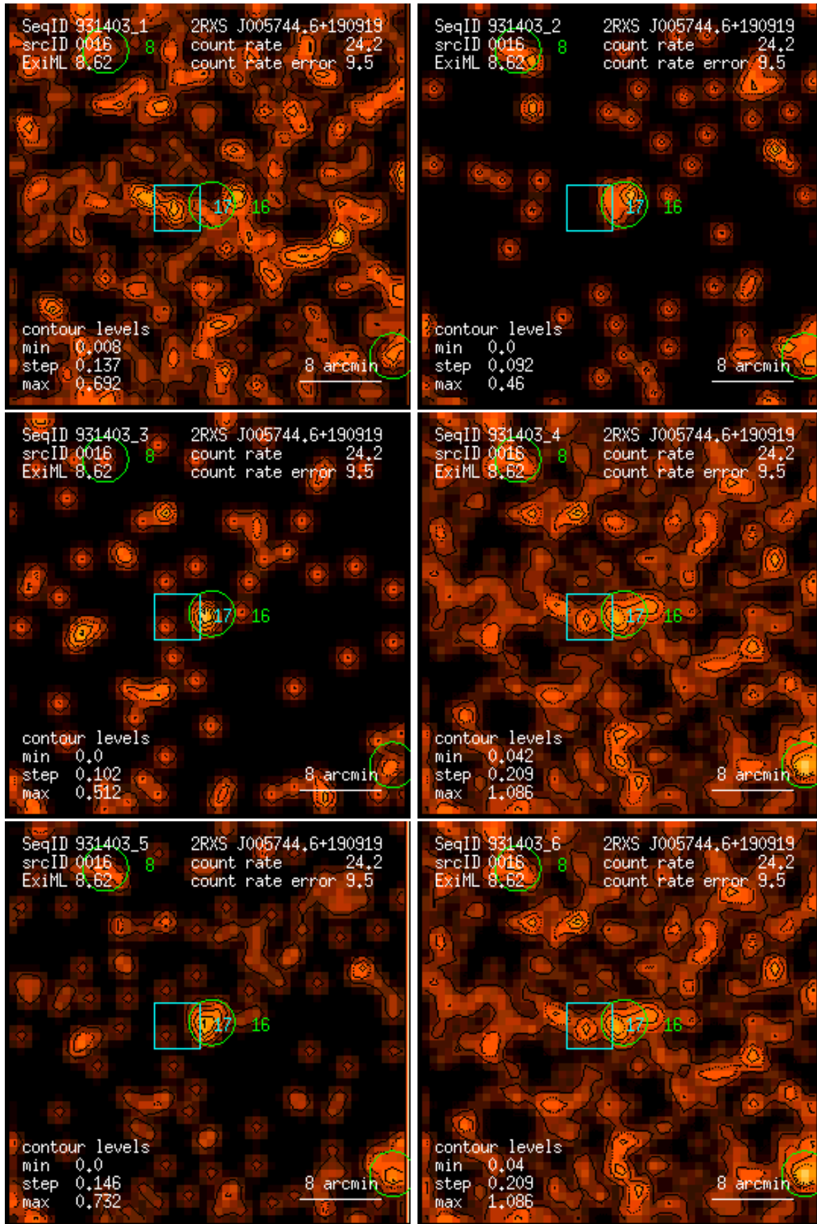
Figure 16: RASS 931403: detection 0016: band rate images, Gaussian filter: (1) PSPC channels 11 – 41, (2) 52 – 90, (3) 91 – 201, (4) 11 – 235, (5) 52 – 201, (6) 11 – 201. Broad band rates in counts/ks. Band rate contour levels in counts/ks/arcmin 2 .
