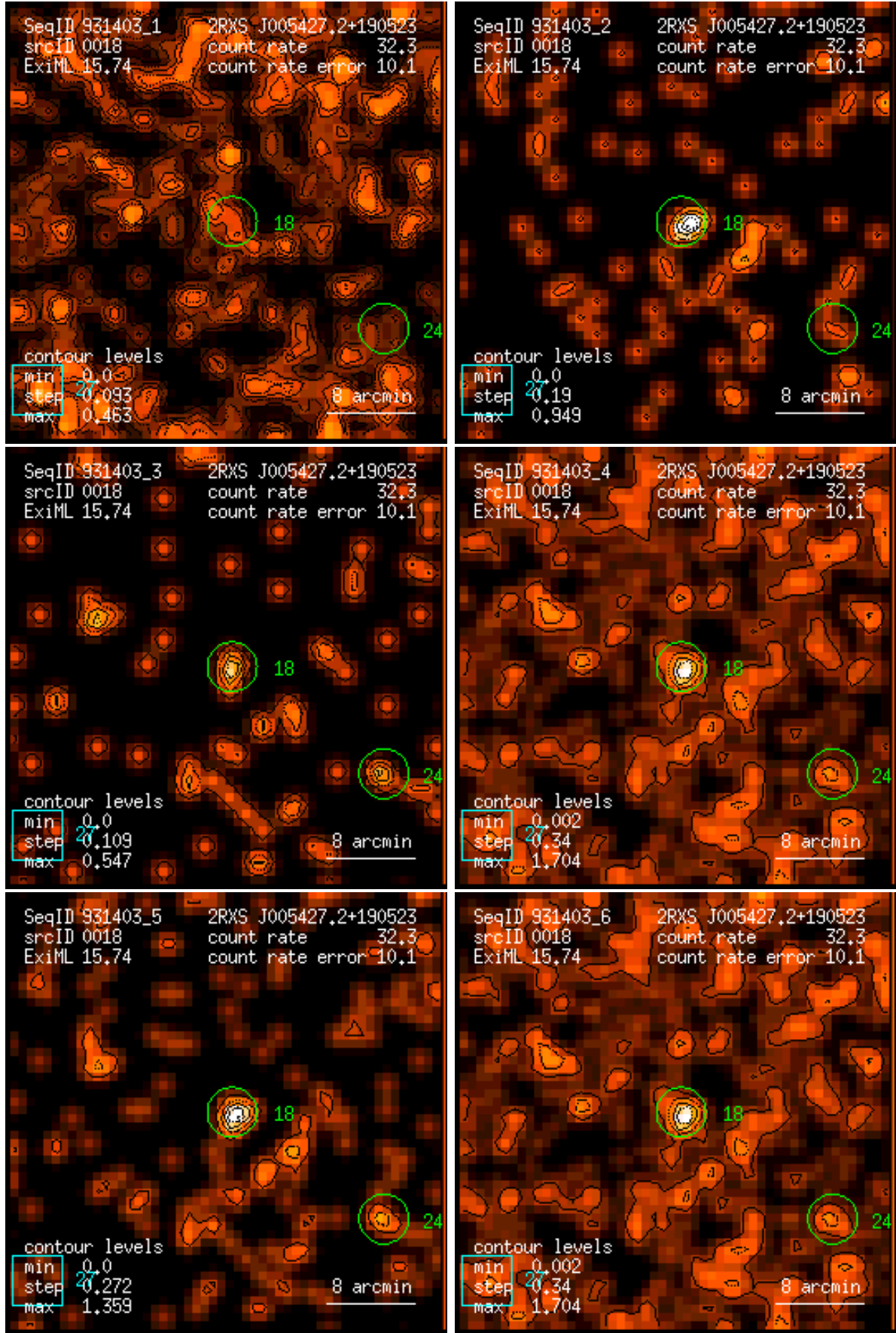
Figure 18: RASS 931403: detection 0018: band rate images, Gaussian filter: (1) PSPC channels 11 – 41, (2) 52 – 90, (3) 91 – 201, (4) 11 – 235, (5) 52 – 201, (6) 11 – 201. Broad band rates in counts/ks. Band rate contour levels in counts/ks/arcmin 2 .
