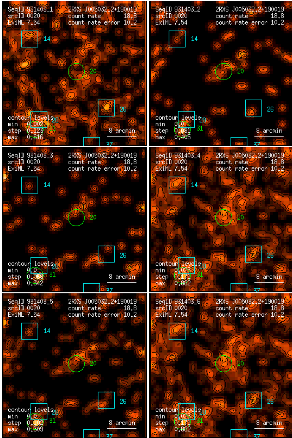
Figure 20: RASS 931403: detection 0020: band rate images, Gaussian filter: (1) PSPC channels 11 – 41, (2) 52 – 90, (3) 91 – 201, (4) 11 – 235, (5) 52 – 201, (6) 11 – 201. Broad band rates in counts/ks. Band rate contour levels in counts/ks/arcmin 2 .
