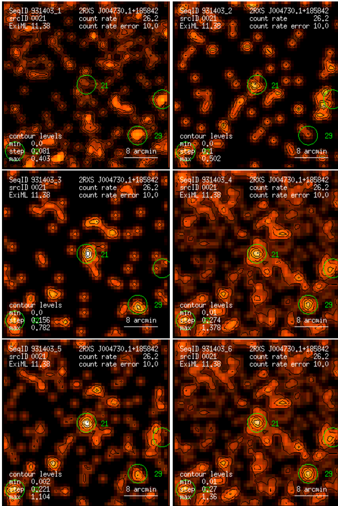
Figure 21: RASS 931403: detection 0021: band rate images, Gaussian filter: (1) PSPC channels 11 – 41, (2) 52 – 90, (3) 91 – 201, (4) 11 – 235, (5) 52 – 201, (6) 11 – 201. Broad band rates in counts/ks. Band rate contour levels in counts/ks/arcmin 2 .
