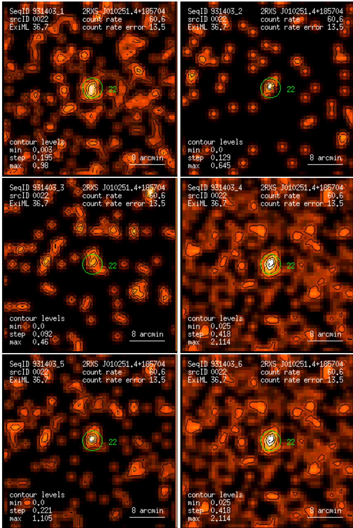
Figure 22: RASS 931403: detection 0022: band rate images, Gaussian filter: (1) PSPC channels 11 – 41, (2) 52 – 90, (3) 91 – 201, (4) 11 – 235, (5) 52 – 201, (6) 11 – 201. Broad band rates in counts/ks. Band rate contour levels in counts/ks/arcmin 2 .
