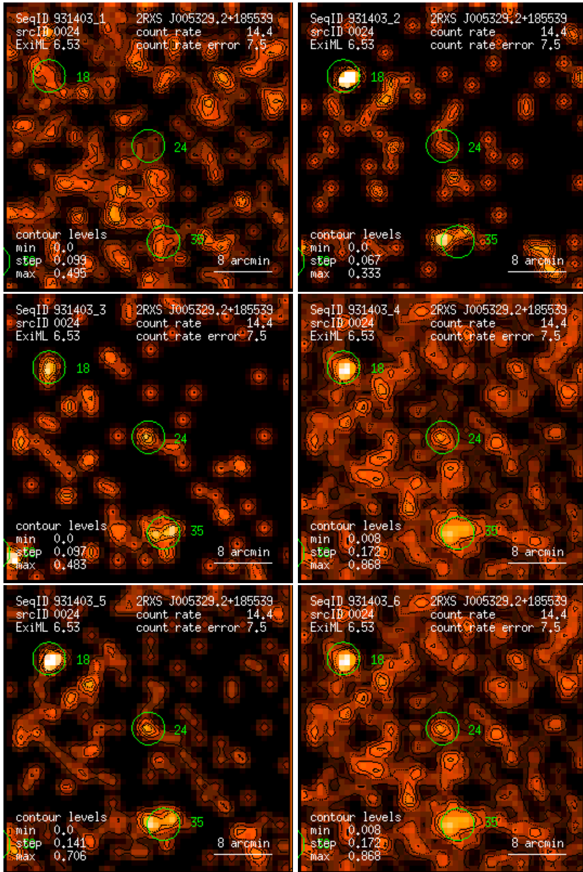
Figure 24: RASS 931403: detection 0024: band rate images, Gaussian filter: (1) PSPC channels 11 – 41, (2) 52 – 90, (3) 91 – 201, (4) 11 – 235, (5) 52 – 201, (6) 11 – 201. Broad band rates in counts/ks. Band rate contour levels in counts/ks/arcmin 2 .
