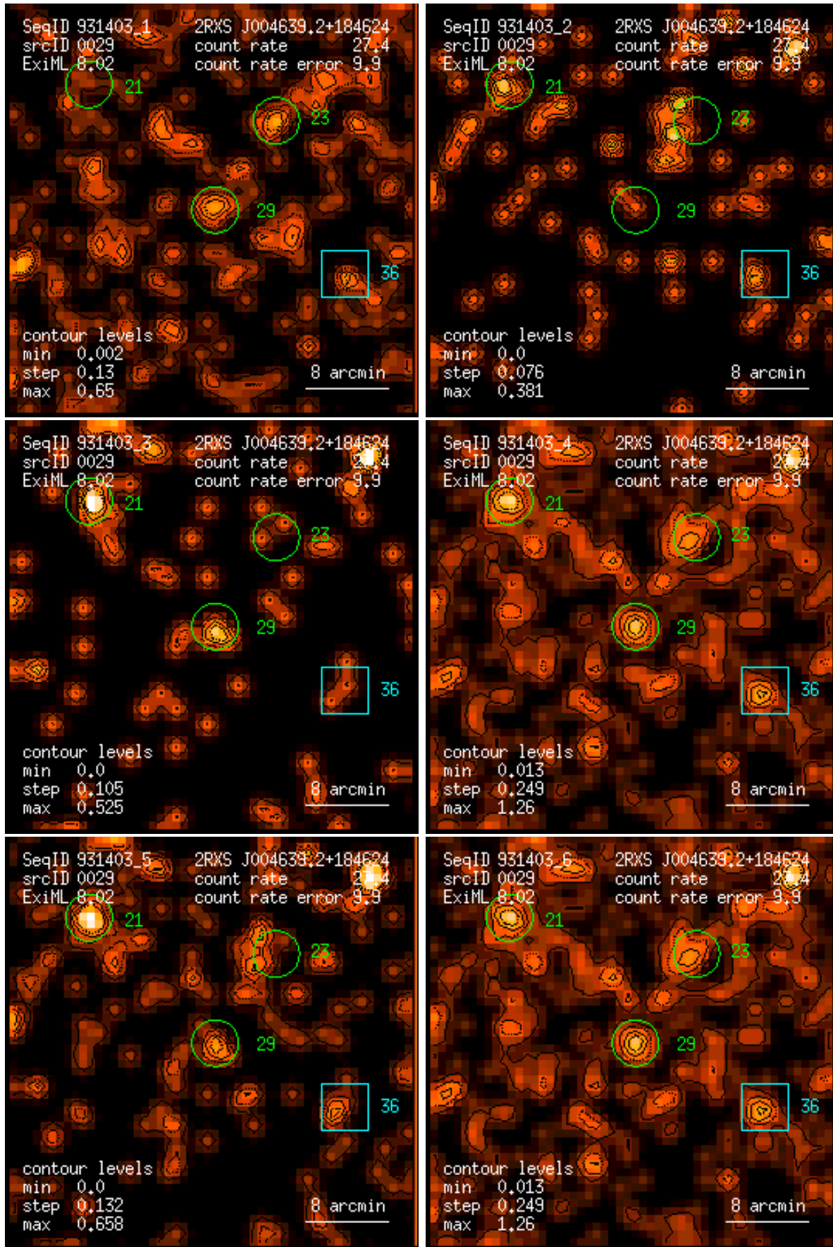
Figure 29: RASS 931403: detection 0029: band rate images, Gaussian filter: (1) PSPC channels 11 – 41, (2) 52 – 90, (3) 91 – 201, (4) 11 – 235, (5) 52 – 201, (6) 11 – 201. Broad band rates in counts/ks. Band rate contour levels in counts/ks/arcmin 2 .
