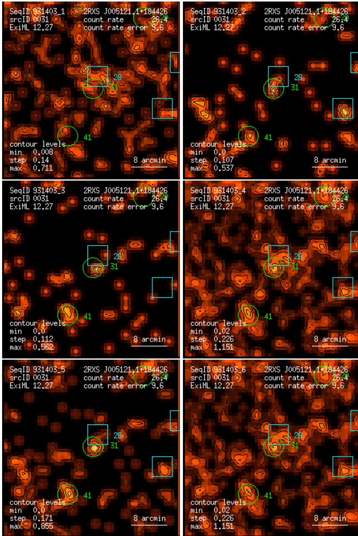
Figure 31: RASS 931403: detection 0031: band rate images, Gaussian filter: (1) PSPC channels 11 – 41, (2) 52 – 90, (3) 91 – 201, (4) 11 – 235, (5) 52 – 201, (6) 11 – 201. Broad band rates in counts/ks. Band rate contour levels in counts/ks/arcmin 2 .
