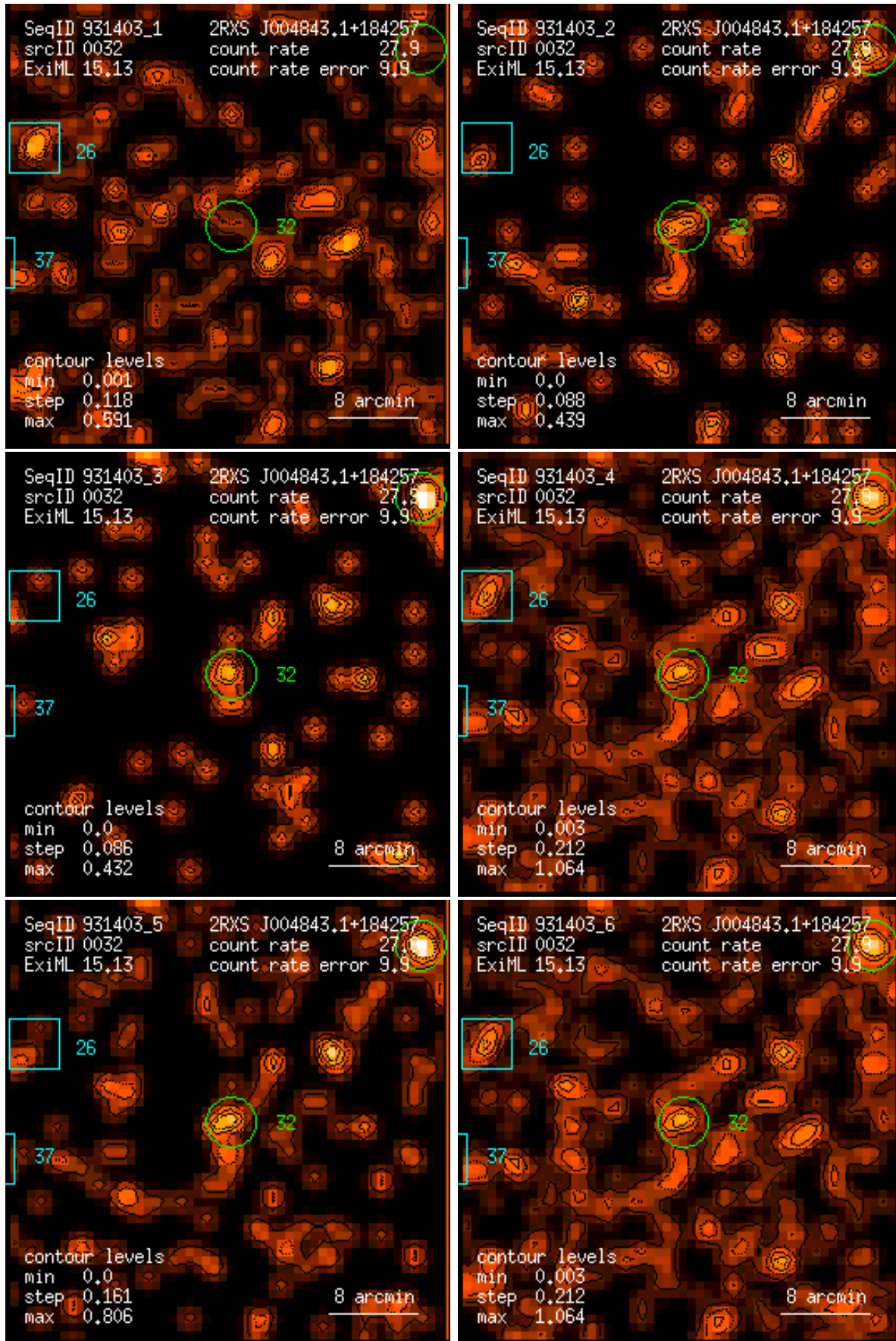
Figure 32: RASS 931403: detection 0032: band rate images, Gaussian filter: (1) PSPC channels 11 – 41, (2) 52 – 90, (3) 91 – 201, (4) 11 – 235, (5) 52 – 201, (6) 11 – 201. Broad band rates in counts/ks. Band rate contour levels in counts/ks/arcmin 2 .
