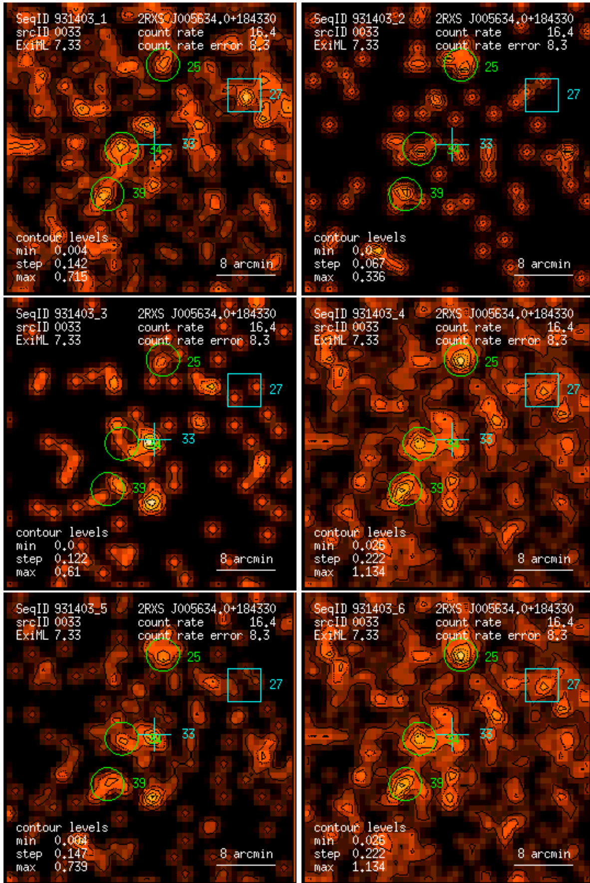
Figure 33: RASS 931403: detection 0033: band rate images, Gaussian filter: (1) PSPC channels 11 – 41, (2) 52 – 90, (3) 91 – 201, (4) 11 – 235, (5) 52 – 201, (6) 11 – 201. Broad band rates in counts/ks. Band rate contour levels in counts/ks/arcmin 2 .
