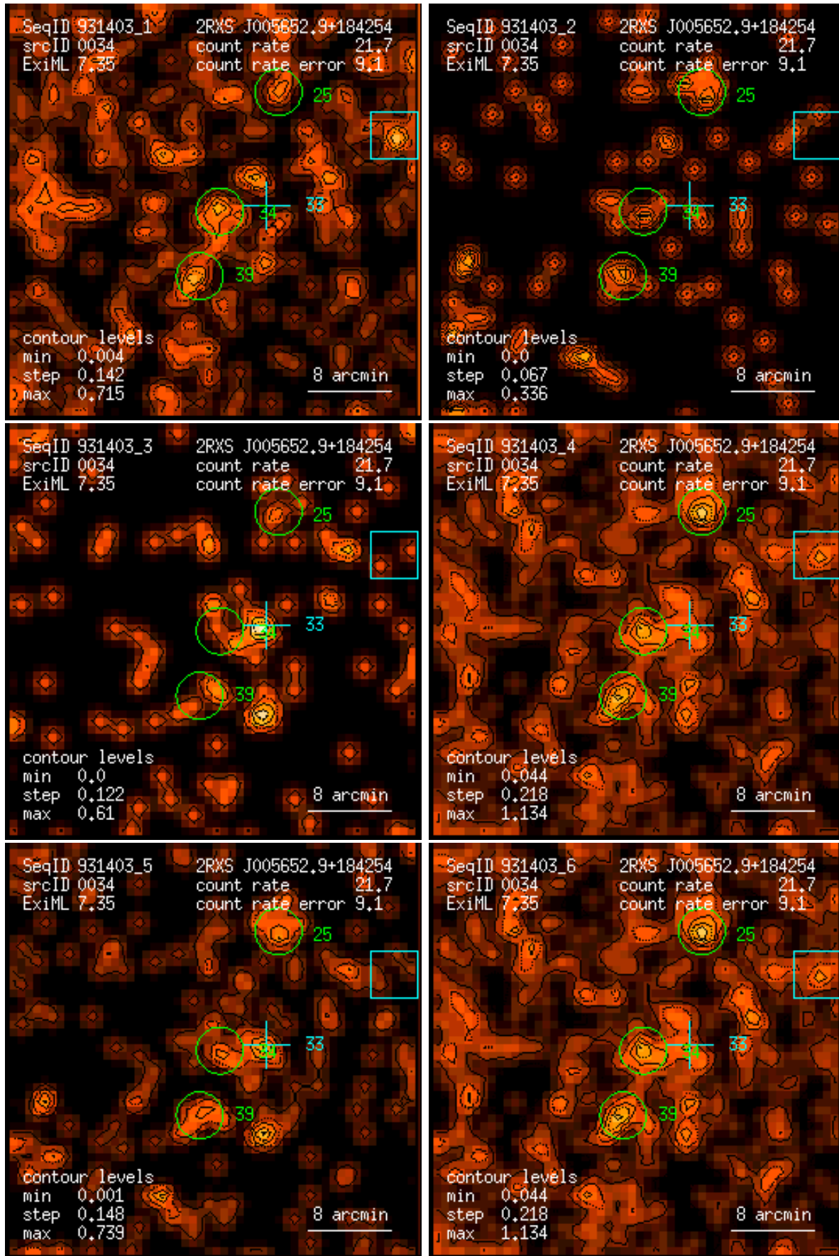
Figure 34: RASS 931403: detection 0034: band rate images, Gaussian filter: (1) PSPC channels 11 – 41, (2) 52 – 90, (3) 91 – 201, (4) 11 – 235, (5) 52 – 201, (6) 11 – 201. Broad band rates in counts/ks. Band rate contour levels in counts/ks/arcmin 2 .
