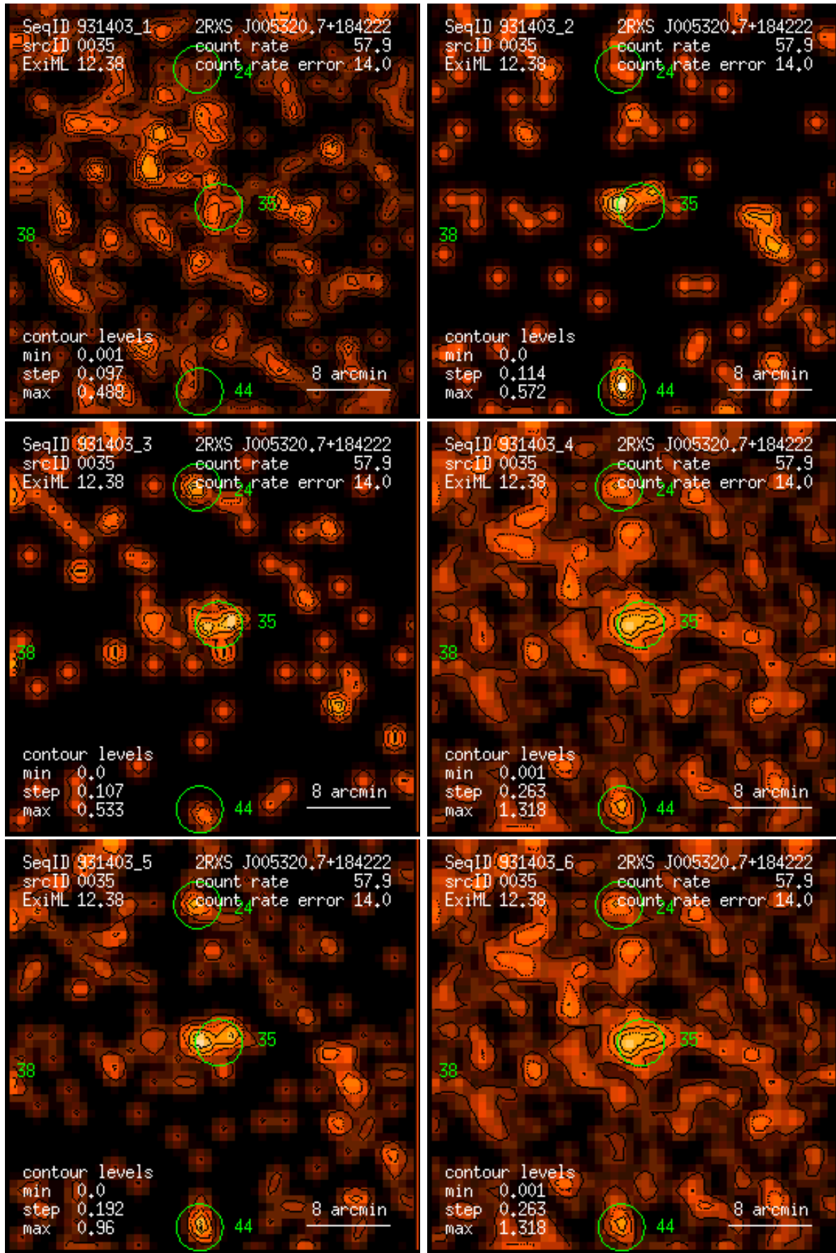
Figure 35: RASS 931403: detection 0035: band rate images, Gaussian filter: (1) PSPC channels 11 – 41, (2) 52 – 90, (3) 91 – 201, (4) 11 – 235, (5) 52 – 201, (6) 11 – 201. Broad band rates in counts/ks. Band rate contour levels in counts/ks/arcmin 2 .
