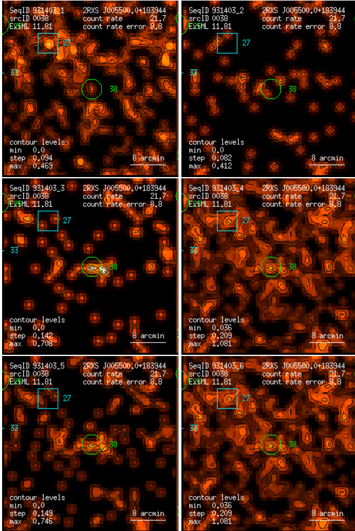
Figure 38: RASS 931403: detection 0038: band rate images, Gaussian filter: (1) PSPC channels 11 – 41, (2) 52 – 90, (3) 91 – 201, (4) 11 – 235, (5) 52 – 201, (6) 11 – 201. Broad band rates in counts/ks. Band rate contour levels in counts/ks/arcmin 2 .
