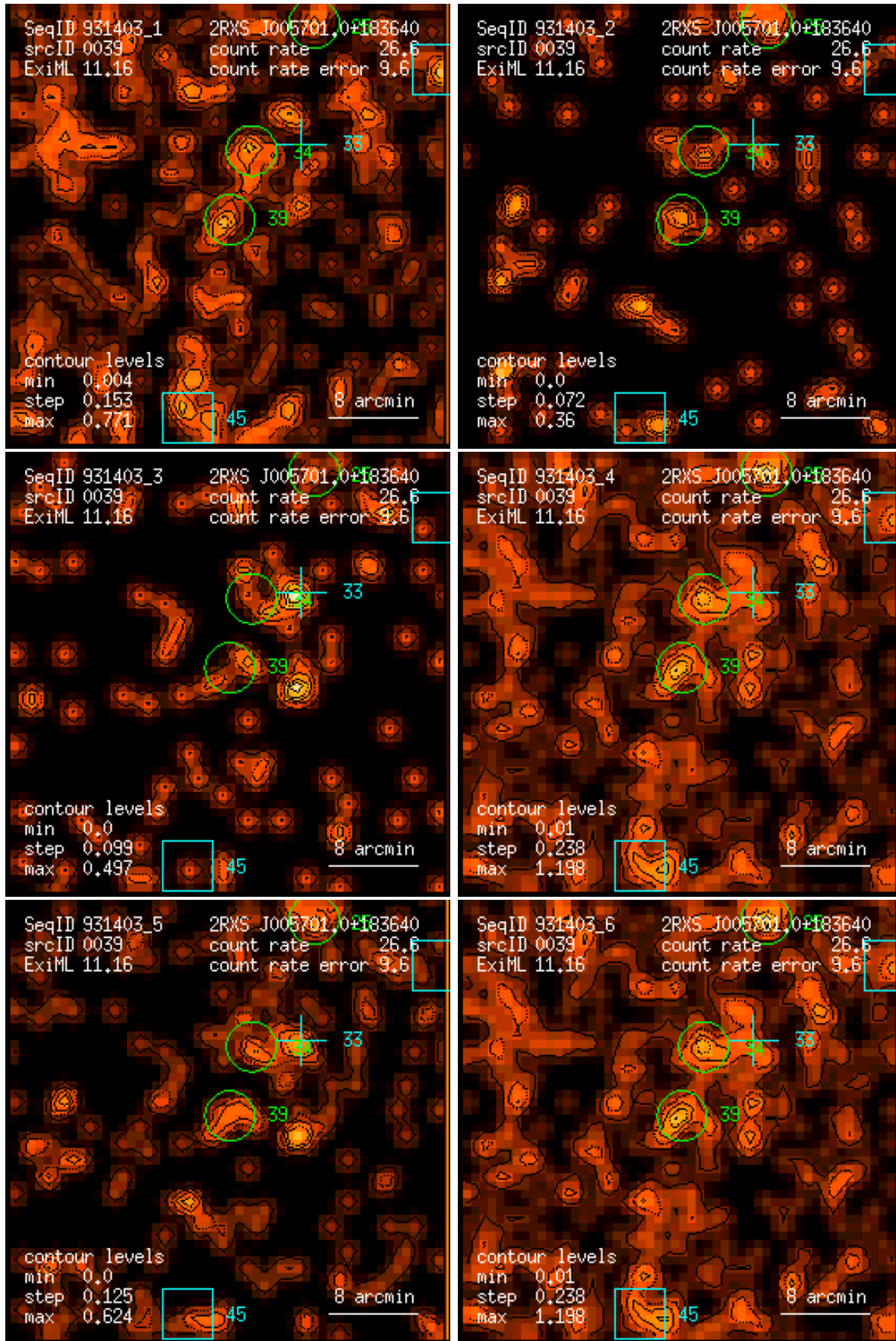
Figure 39: RASS 931403: detection 0039: band rate images, Gaussian filter: (1) PSPC channels 11 – 41, (2) 52 – 90, (3) 91 – 201, (4) 11 – 235, (5) 52 – 201, (6) 11 – 201. Broad band rates in counts/ks. Band rate contour levels in counts/ks/arcmin 2 .
