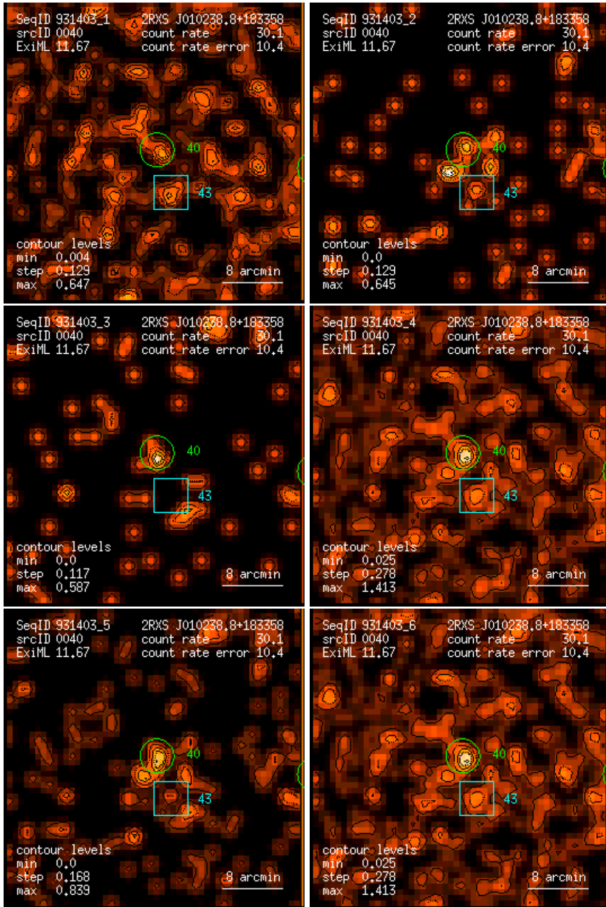
Figure 40: RASS 931403: detection 0040: band rate images, Gaussian filter: (1) PSPC channels 11 – 41, (2) 52 – 90, (3) 91 – 201, (4) 11 – 235, (5) 52 – 201, (6) 11 – 201. Broad band rates in counts/ks. Band rate contour levels in counts/ks/arcmin 2 .
