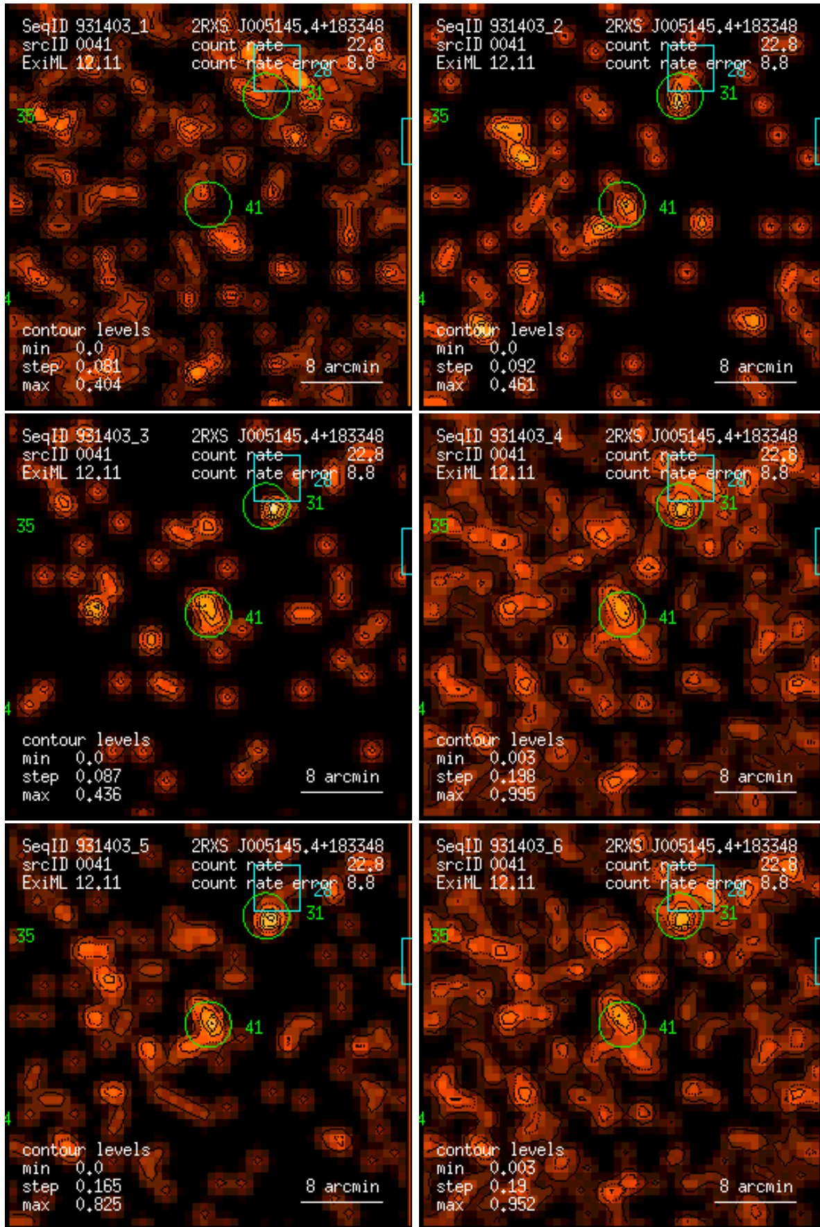
Figure 41: RASS 931403: detection 0041: band rate images, Gaussian filter: (1) PSPC channels 11 – 41, (2) 52 – 90, (3) 91 – 201, (4) 11 – 235, (5) 52 – 201, (6) 11 – 201. Broad band rates in counts/ks. Band rate contour levels in counts/ks/arcmin 2 .
