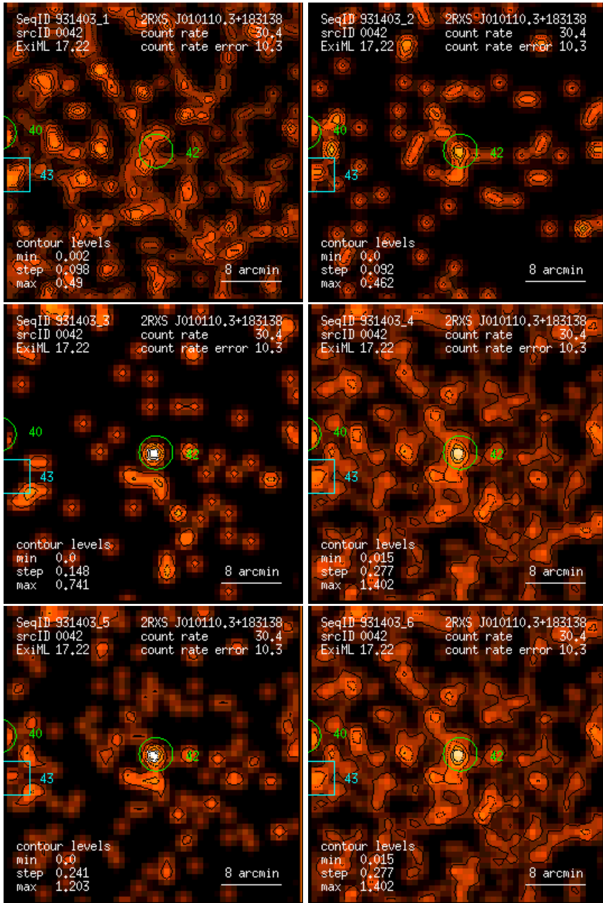
Figure 42: RASS 931403: detection 0042: band rate images, Gaussian filter: (1) PSPC channels 11 – 41, (2) 52 – 90, (3) 91 – 201, (4) 11 – 235, (5) 52 – 201, (6) 11 – 201. Broad band rates in counts/ks. Band rate contour levels in counts/ks/arcmin 2 .
