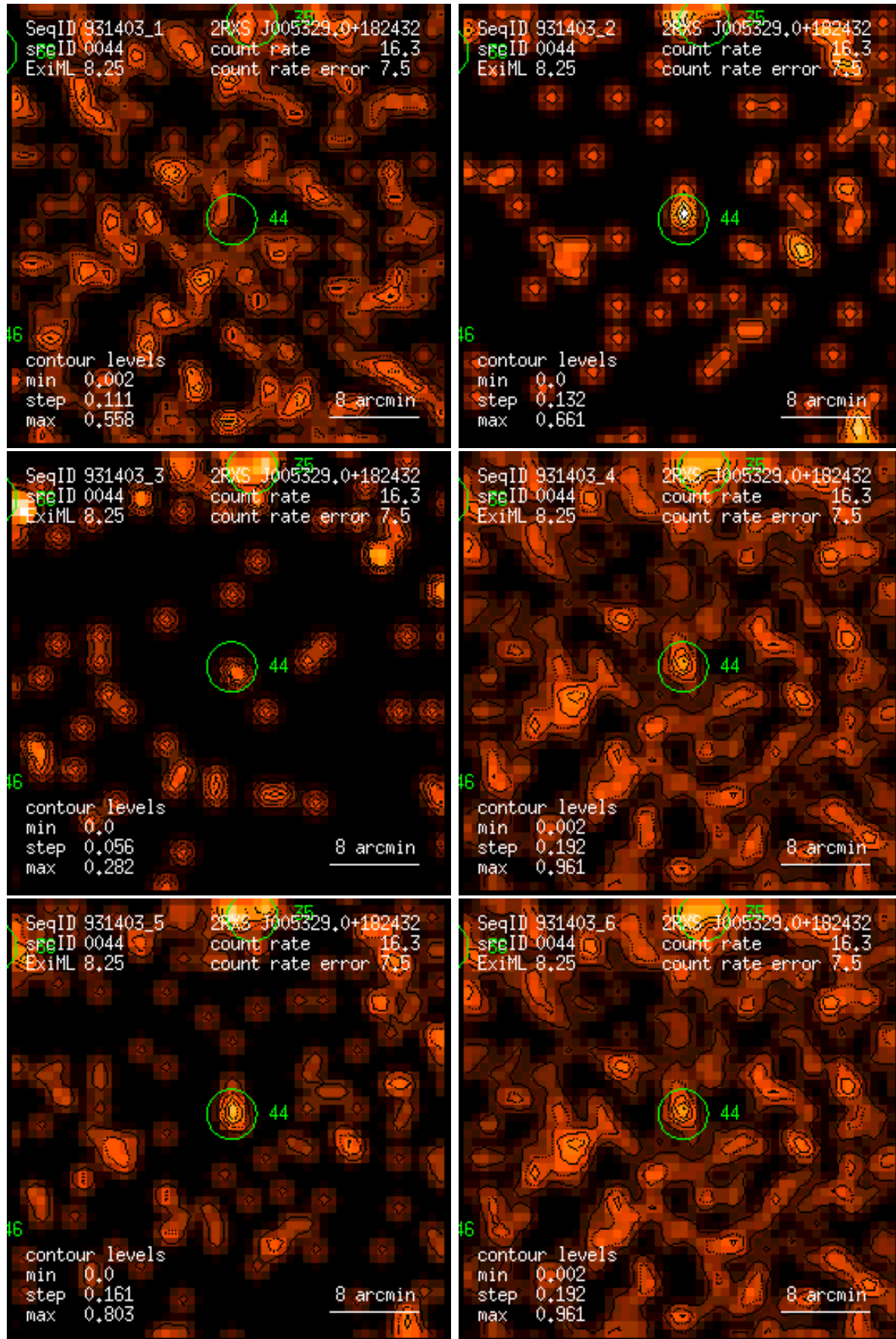
Figure 44: RASS 931403: detection 0044: band rate images, Gaussian filter: (1) PSPC channels 11 – 41, (2) 52 – 90, (3) 91 – 201, (4) 11 – 235, (5) 52 – 201, (6) 11 – 201. Broad band rates in counts/ks. Band rate contour levels in counts/ks/arcmin 2 .
