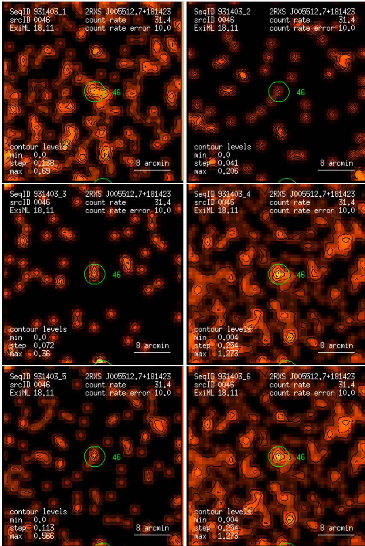
Figure 46: RASS 931403: detection 0046: band rate images, Gaussian filter: (1) PSPC channels 11 – 41, (2) 52 – 90, (3) 91 – 201, (4) 11 – 235, (5) 52 – 201, (6) 11 – 201. Broad band rates in counts/ks. Band rate contour levels in counts/ks/arcmin 2 .
