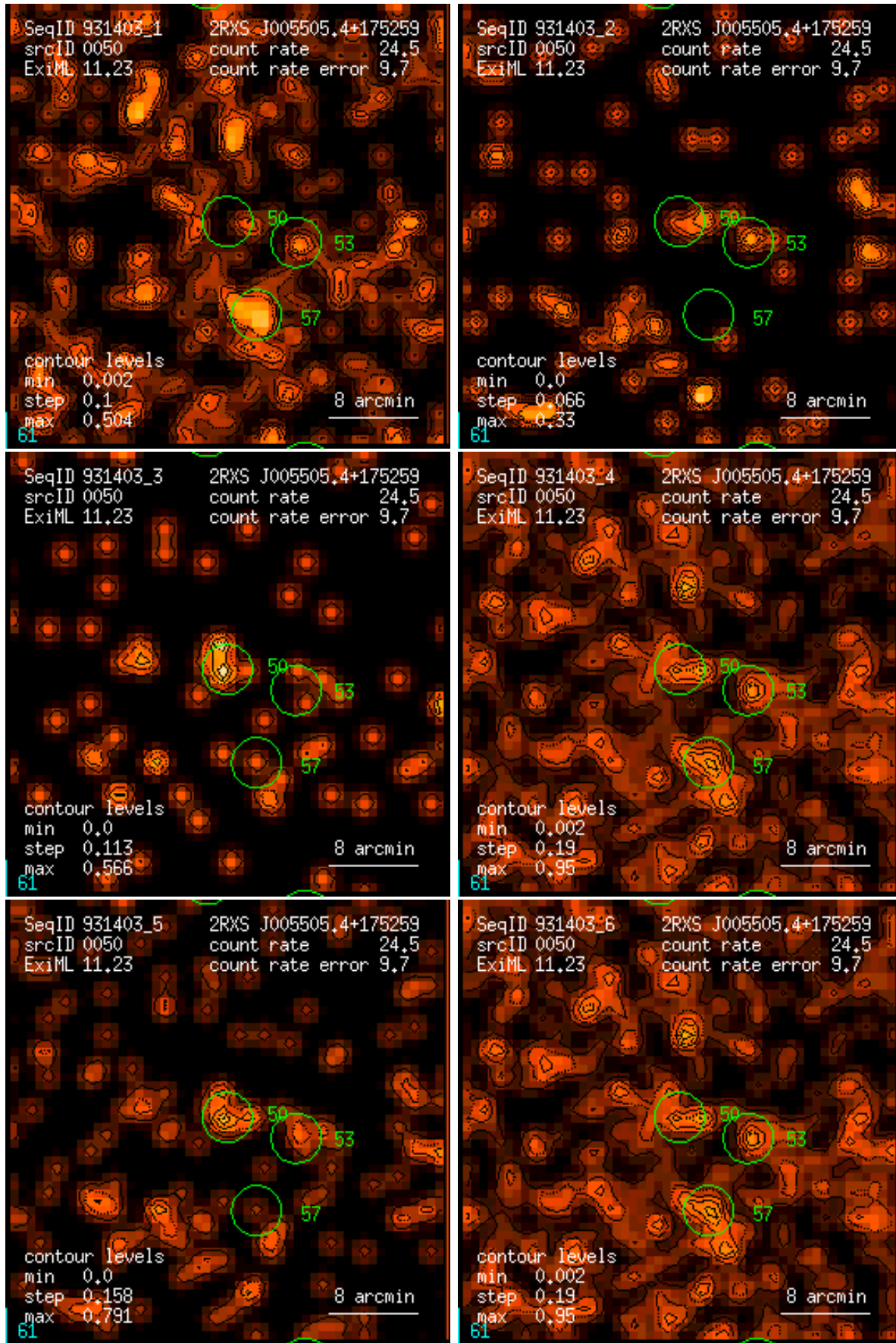
Figure 50: RASS 931403: detection 0050: band rate images, Gaussian filter: (1) PSPC channels 11 – 41, (2) 52 – 90, (3) 91 – 201, (4) 11 – 235, (5) 52 – 201, (6) 11 – 201. Broad band rates in counts/ks. Band rate contour levels in counts/ks/arcmin 2 .
